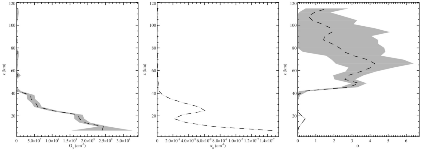
Fig. 14. Same as Fig. 12 for NOMAD-UVIS occultation observation obtained on June 21, 2018, at 0809 UT. (Standard UVIS data ID: nmd_cal_sc_uv-is_20180621T080914-20,180,621 T082453-i).
