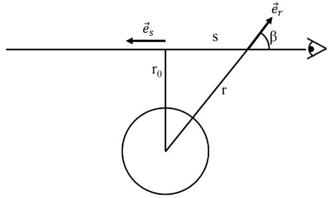
Fig. 1. Line-of-sight integration geometry. Variable s measures location along the line-of-sight (l.o.s.), from the tangent point located at distance r_0 from the planet center, where the radial direction is perpendicular to the l.o.s.. It is counted positively in the direction of a chosen reference unit vector \vec{e}_s . For a given value of r_0 , angle \beta can also be used to specify the location along the l.o.s., and therefore the value of radial distance r and the orientation of the radial unit vector \vec{e}_r .
