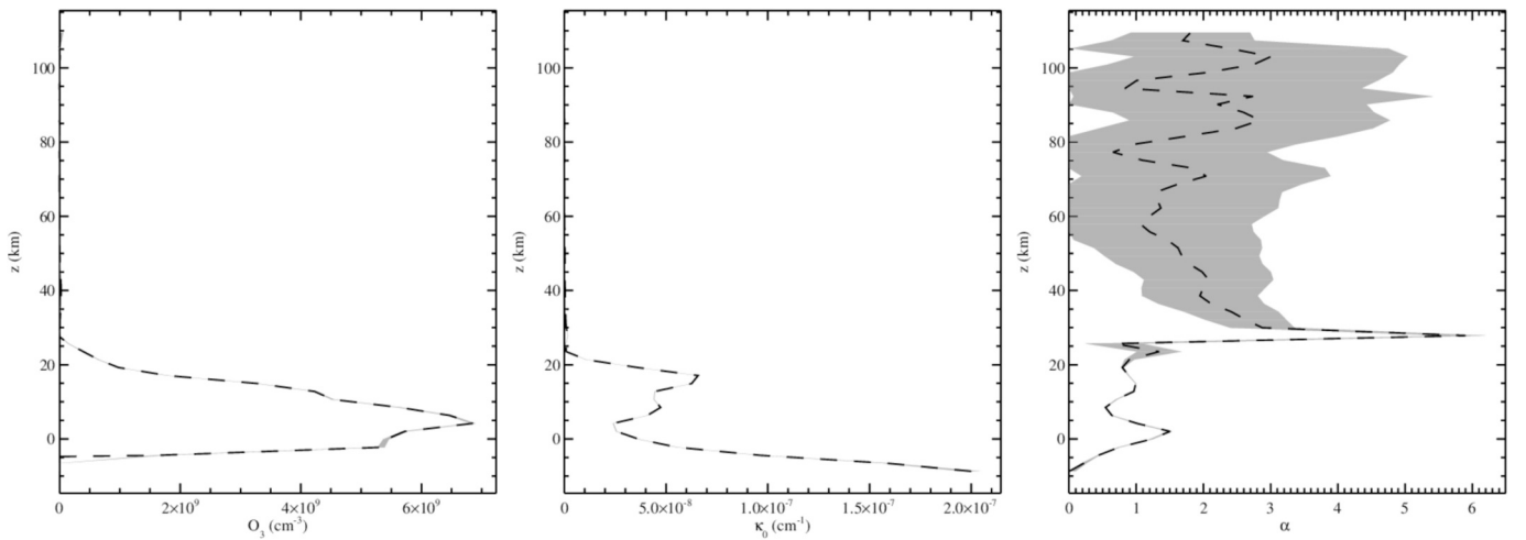
Fig. 12. Results of the inversion of the solar occultation of the Mars atmosphere observed with EXOMARS-NOMAD-UVIS on May 4, 2018, at 0059 UT. The altitude is estimated from a reference radial distance of 3390 km. Grey shades give the 1- \sigma standard deviation over the fitting parameters, i.e., from left to right, the ozone density, the differential extinction parameter of the dusts, and the Angström \alpha parameter of the dusts. (Standard UVIS data ID: nmd_cal_sc_uvvis_20180504T005927-20,180,504 T011659-e).
