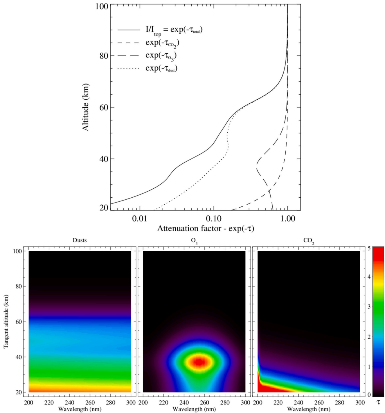
Fig. 3. Attenuation of the solar radiation at 285 nm as a function of tangent point altitude, under occultation through the Mars atmosphere, simulated using the atmosphere characteristics shown in Fig. 2 (top panel). The contributions of the dusts, CO 2 and O 3 are explicitly given. Local extremum of an absorber can lead to a local minimum in the attenuation factor vertical profile. Attenuation optical thickness of the dusts, ozone and CO 2 in the 200–300 wavelength range for lines of sights having their tangent height ranging from 20 to 100 km (bottom panels).
