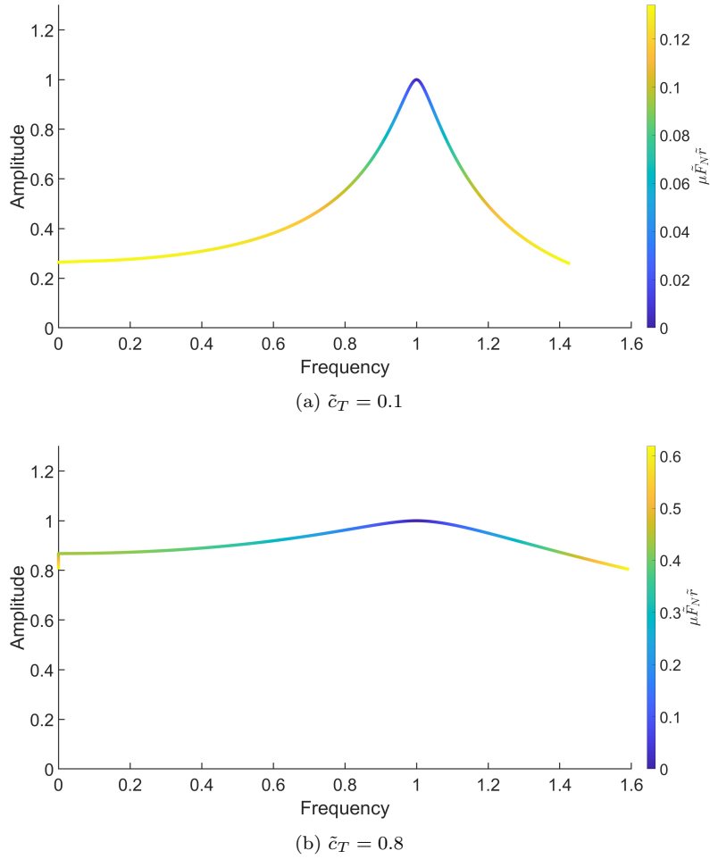
Figure 22: Enlargement of the stick limit boundaries with \mu\tilde{F}_N . Limit amplitude against limit frequency for different values of \tilde{c}_T under the constat clamp motion amplitude of 0.001.
