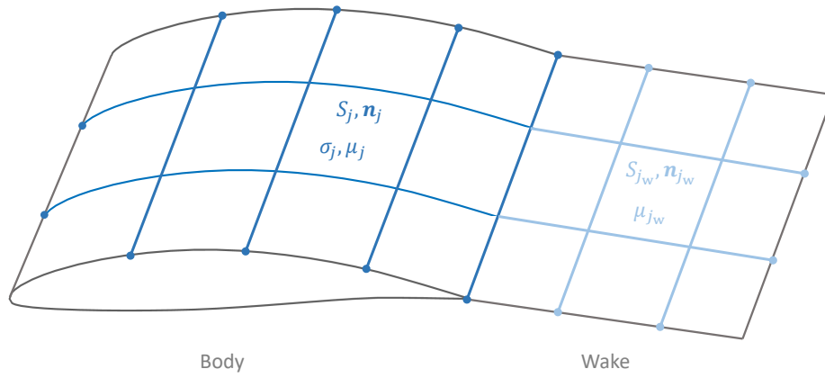
Figure 2.1: Discretized geometry with panel of surface area S , unit normal \mathbf{n} , sources \sigma and doublets \mu .
