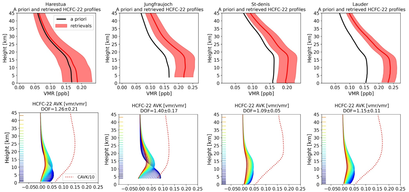
Figure 2. Top panels: The a priori and retrieved HCFC-22 profiles (mean and SD) at Harestua, Jungfrauoch, St-Denis and Lauder. Bottom panels: The profile averaging kernel matrix (AVK) and column averaging kernel vector (CAVK).
