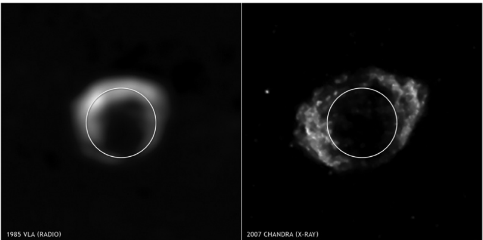
1985 VLA (RADIO)
