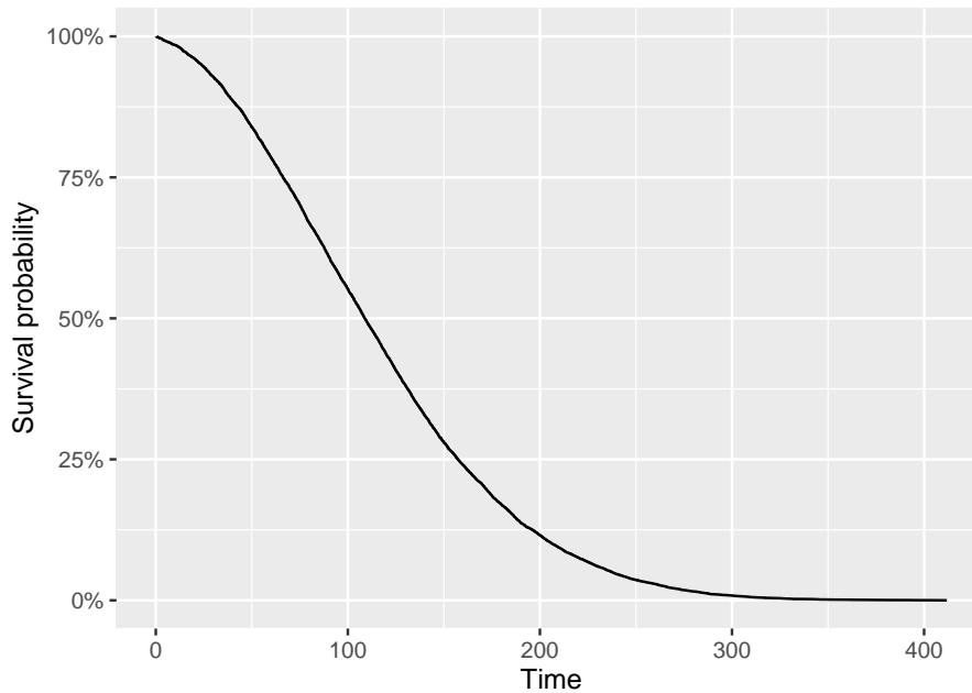
Figure 1.2: Example of a survival function S(t)
