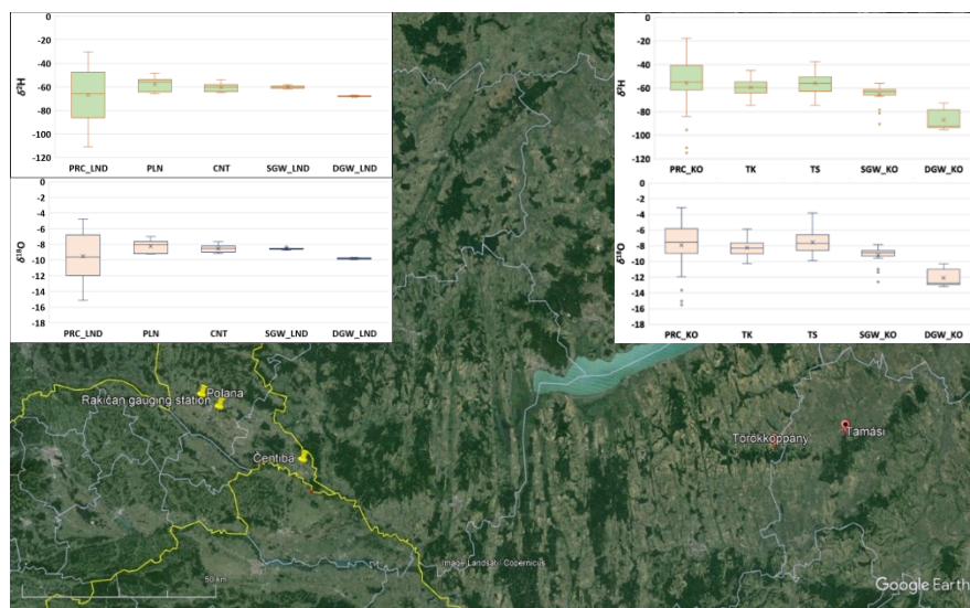
Figure 1: Location of studies catchments and monitoring sites in Hungary (Törökkoppány (TK) and Tamási (TS), red markers) and Slovenia (Rakičan (LND), Čentiba (CNT) and Polana (PLN), yellow markers). Box-and-whiskers plots of precipitation-river-subsurface water (shallow (SGW) and deep (DGW) at the sites are shown for the Ledava catchment (SI, left) and the Koppány catchment (HU, right). Basemap from Google Earth.
