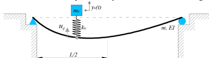
Figure 1. Structural diagram of the vehicle-bridge interacting system.
