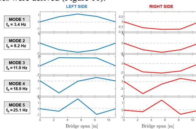
Figure 11. Modal shapes related to the first five frequencies of the bridge (VBI-based procedure).
