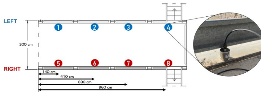
Figure 3. Position of the accelerometers on the deck and a picture of one of the sensors.
