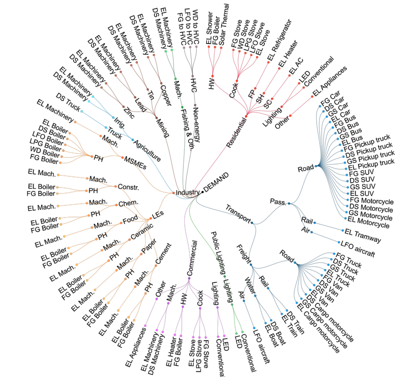
Figure 1: Radial tree representation of the energy demand model. The abbreviations are: DS: Diesel, EL: Electricity, FG: Fossil gas, GS: Gasoline, HW: Hot Water, Irrig: Irrigation, LES: Large enterprises, LFO: Light fuel oil, LPG: Liquefied petroleum gas, Mach: Machinery, MSMEs: Micro, small and medium-sized enterprises, Pass: Passenger, PH: Process Heat, SUV: Sport utility vehicle, WD: Biomass, Fishing & Oth.: Fishing & Others, HVC: High Value Chemicals.
