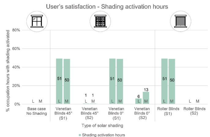
Fig. 13. Comparison of shadings activation hours during working hours. Case of Liège (L) and Milan (M).
