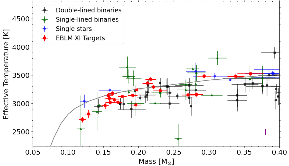
Figure 5. A cutout of the stellar mass versus effective temperature diagram using results from Nefs et al. (2013); Gillen et al. (2017); Parsons et al. (2018); Jennings et al. (2023); Duck et al. (2023); Martin et al. (2023), with our results highlighted in red. The type of system is displayed by different colours. The theoretical relation from Baraffe et al. (2015) for an age of 1 Gyr is plotted in gray. The systematic error of 50 K that is added to our final results has been displayed in the bottom right of the Figure in purple.
