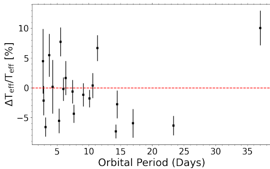
Figure 9. The orbital period of a target versus the percentage effective temperature anomaly (i.e. the percentage change of our observationally derived stellar effective temperature from the theoretical effective temperature).
