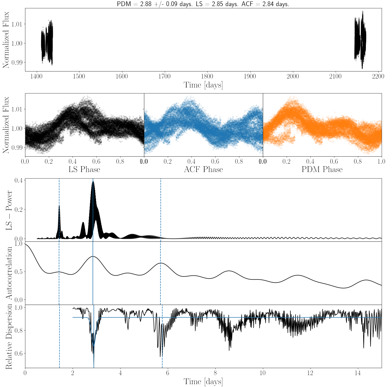
Figure 2. A set of output plots generated by the module STARSPOT when analysing the masked flux signal of EBLM J0239-20. The top plot displays the inputted flux signal. The second shows the flux signal phase folded by the fitted variation period for each method (Lomb-Scargle, autocorrelation functions and phase dispersion minimisation). The third, fourth and fifth plots are the plotted results of each method showing the period versus the signal detection likelihood. In this example Lomb-Scargle periodograms finds a variation signal with a period of 2.85 days, the autocorrelation function finds a variation signal with a period of 2.84 days and the phase dispersion minimisation fits a period of 2.88 days.
