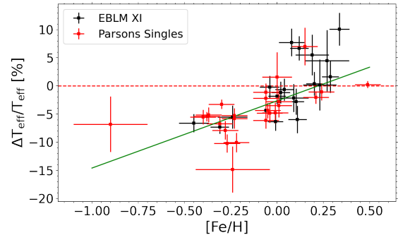
Figure 7. The percentage effective temperature anomaly, versus the target’s metallicity for all our targets and the single object systems in Parsons et al. (2018). A linear fit of the data is plotted over the data in green.
