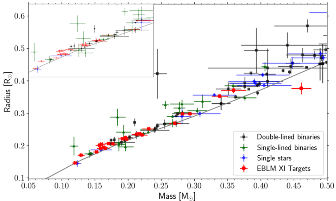
Figure 4. A cutout of the stellar mass versus stellar radius diagram using results from Nefs et al. (2013); Gillen et al. (2017); Parsons et al. (2018); Jennings et al. (2023); Duck et al. (2023); Martin et al. (2023) with our results highlighted in red. The type of system is displayed by different colours. The theoretical relation from Baraffe et al. (2015) for an age of 1 Gyr is plotted in gray.
