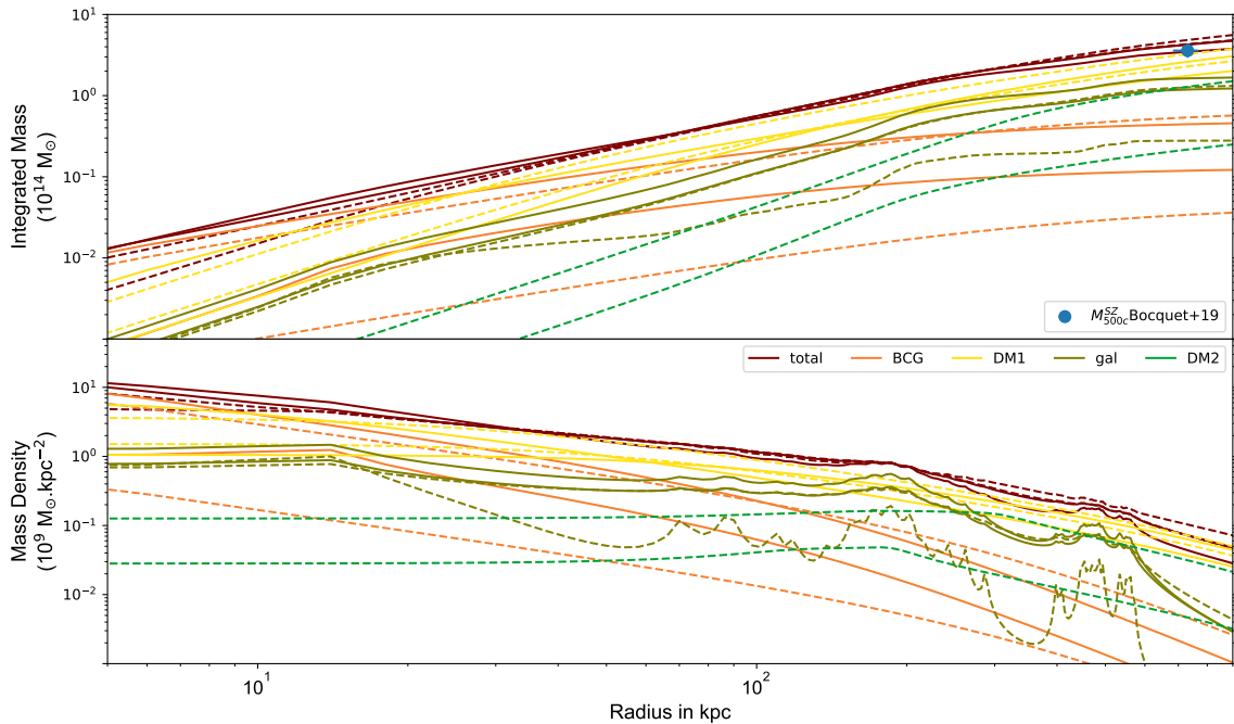
Figure 7. The integrated (upper panel), and differential (lower panel) mass profile of the cluster. The mass profiles are drawn from a circular aperture centered on the BCG. The color coding shows the total mass profiles as well as the different sub-components. The solid and dashed lines represent the set of models with one dark matter halo and two dark matter halos, respectively. The blue dot marks the estimated SZ mass of the cluster from Bocquet et al. (2019).
