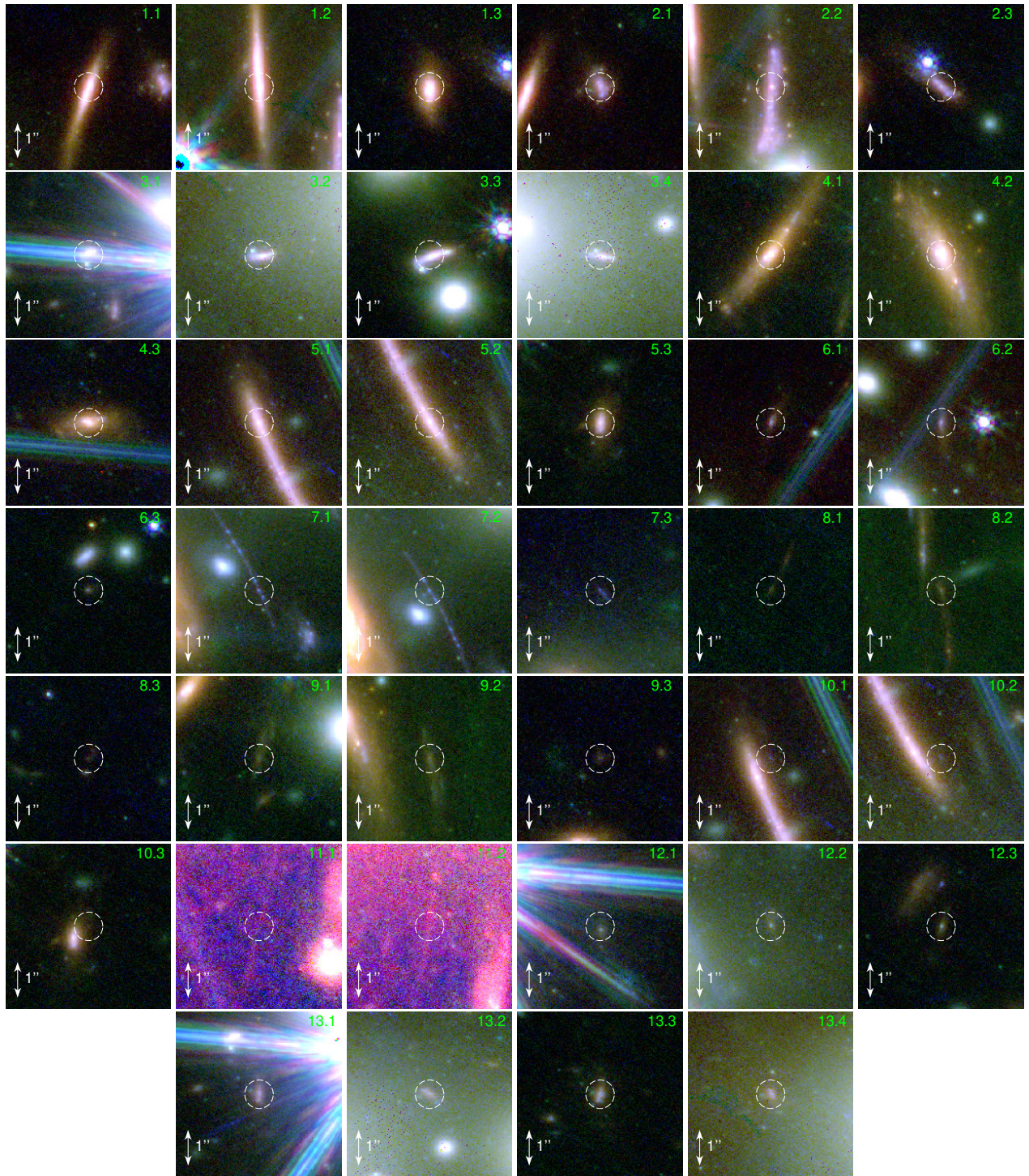
Figure 13. Thumbnails of multiple imaged sources behind SMACS J0723
