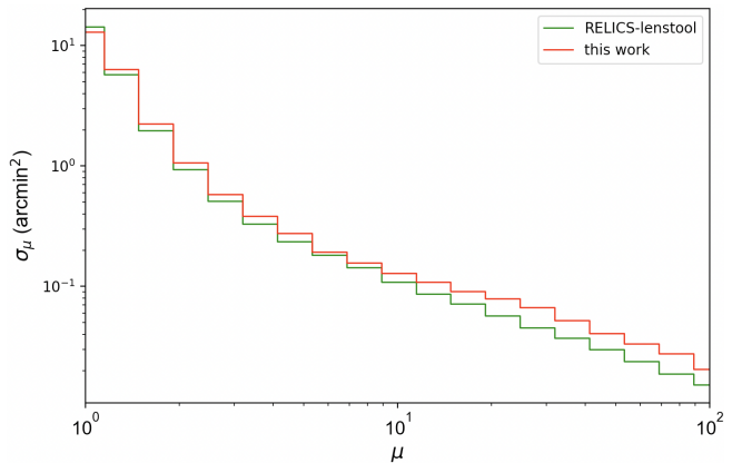
Figure 8. Surface area in the source plane within a 300'' box centered on the cluster at a magnification above a given threshold \mu for a source at z=9 . We here compare the values obtained with our updated mass model with those from the RELICS-LENSTOOL model.
