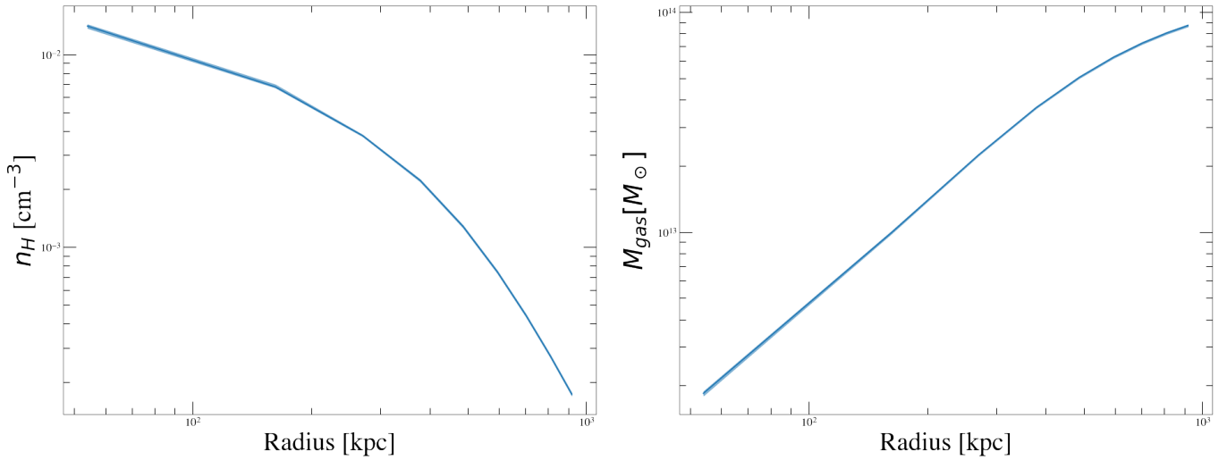
Figure 12. Profiles of the ICM density (left) and the cumulative gas mass (right) as determined from a spherical-deprojection analysis.
