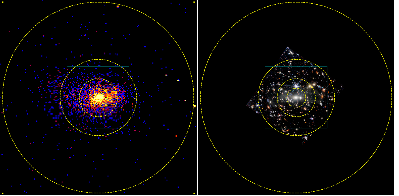
Figure 9. Regions of interest for our measurements of the ICM temperature overlaid on the Chandra ACSI-I image of SMACS J0723 (left; 2'' pixels, 0.5–7 keV, logarithmic intensity scaling) and on the JWST image of the system (right). The dashed circles have radii of 100, 200, 400, and 1000 kpc, respectively, at the cluster redshift. The cyan square marks the region shown in Fig. 1.
