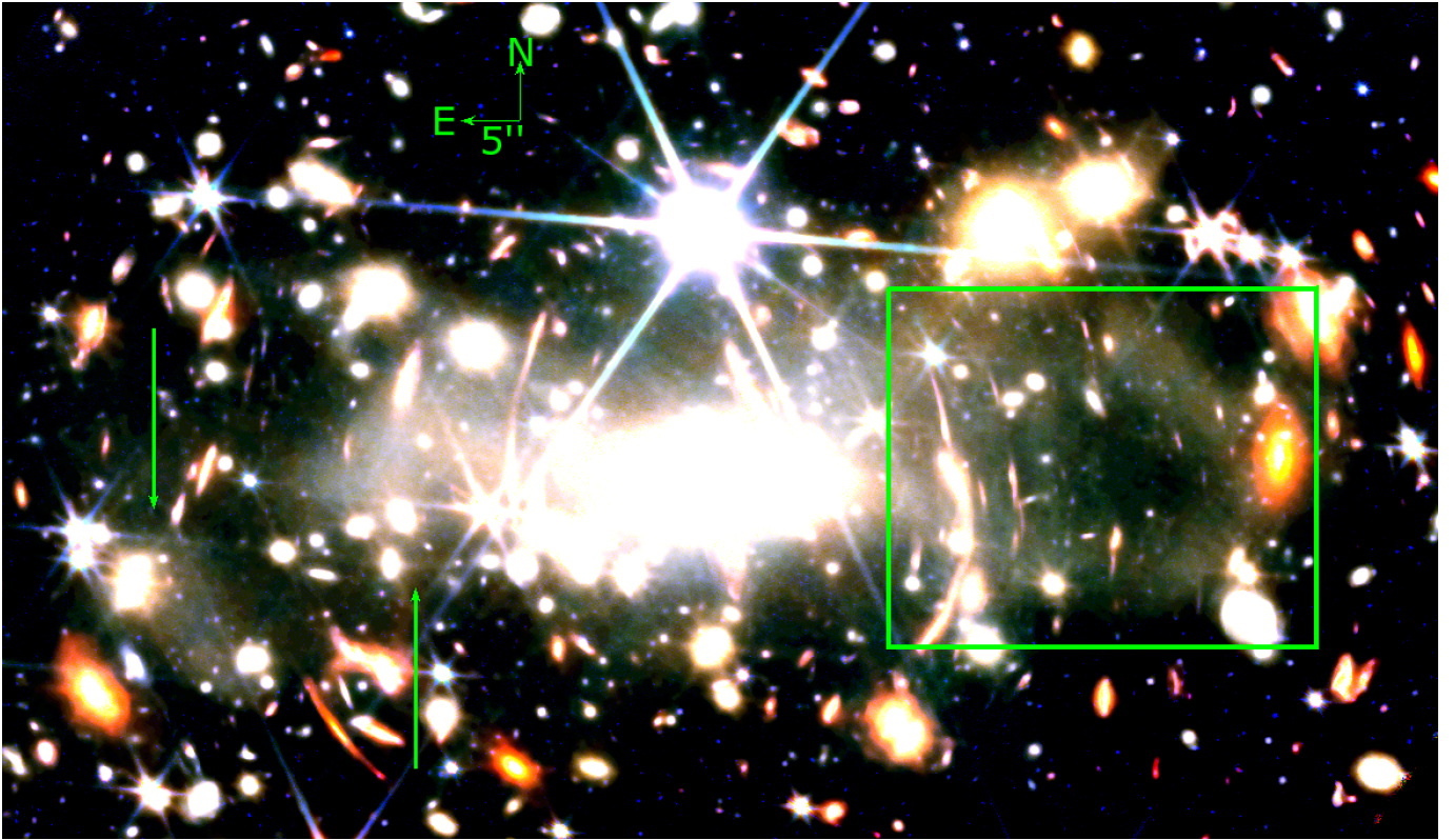
Figure 2. JWST / NIRCam image displayed at high contrast after median filtering with a sliding box spanning 21 \times 21 arcseconds to enhance low-surface-brightness features. Very faint, diffuse emission well beyond the BCG halo is highlighted in a rectangular area west of the cluster core. This image also shows smooth emissions marked by arrows.
