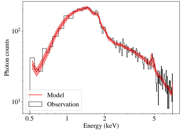
Figure 10. Global spectrum of the observed ICM emission within 1 Mpc of the X-ray peak, corresponding to approximately r_{1000} , (the radius enclosing a thousand times the mean density of the universe at that redshift). Overlaid in red is the best-fit APEC model with its associated 68% confidence range.
