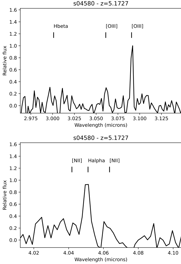
Figure 5. Identified emission lines in the NIRSpect/G395m spectrum of image 7.1. The detection of strong [OIII]5007Å and H \alpha lines, accompanied by weaker [OIII]4959Å and [NII] emission, makes this redshift determination robust.
