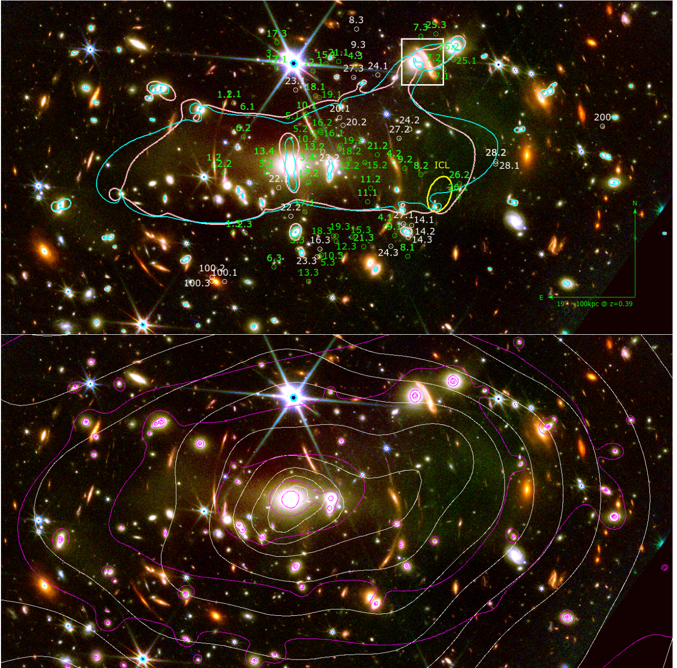
Figure 4. Top: Color image of SMACS J0723 with multiple-image systems used in our models marked by green circles and all other candidates marked as white circles. Also shown are the critical curves for a source at redshift z = 9 ; in cyan for the single-component lens model and in pink for our final model that includes one additional mass clump marked by excess ICL at the location of the yellow ellipse. The white square highlights the 'Beret' galaxy, a highly stretched spiral at z = 1.16 that is only partly multiply imaged (Sect. 5.3). Bottom: Color image of SMACS J0723 with mass contours (in magenta) and X-ray surface-brightness contours (in white) overlaid. We note the visual similarity in ellipticity and asymmetrical distribution along the East-West axis.
