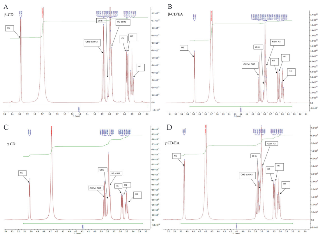
Figure 4 : (A) ^1\text{H} -NMR spectra of \beta -CD, (B) EA- \beta -CD complex in \text{D}_2\text{O} at 25^\circ\text{C} and (C) \gamma CD and (D) EA- \gamma CD complex in \text{D}_2\text{O} at 25^\circ\text{C}
