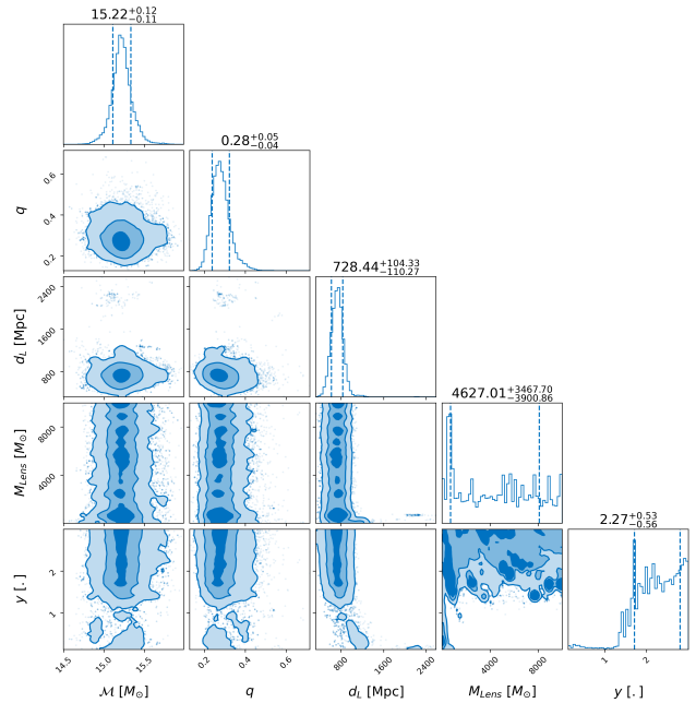
Figure 3. Posteriors for a subset of the parameters including the detector frame chirp mass and mass ratio, the luminosity distance, the lens frame lens mass, and the dimensionless displacement of the source from the optical axis (i.e. the source position). These posteriors were produced during the point mass microlensing analysis done for GW190412 using GRAVELAMPS. As can be seen, similarly to GW191103 (shown in Fig. 8), the lensing parameter posteriors are extremely broad and uninformative. This is consistent with the expectations for a non-microlensing event.
