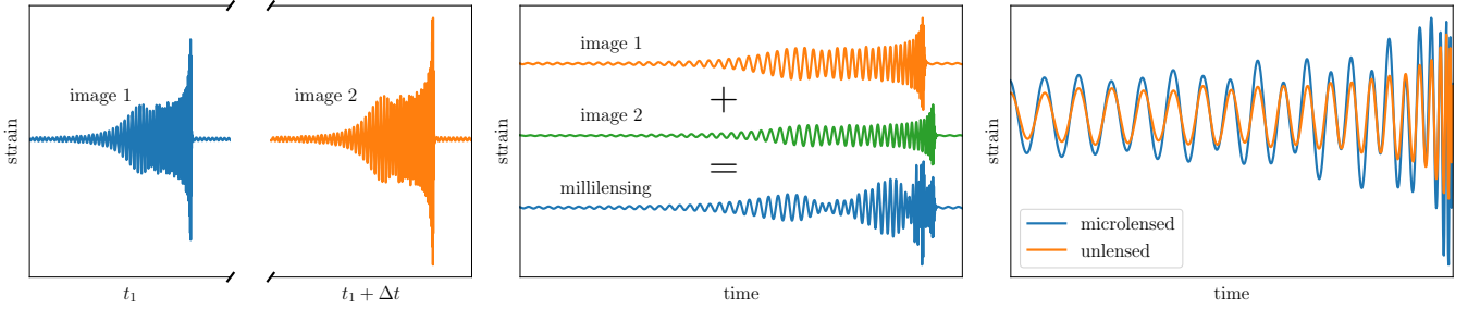
Figure 1. A representation of the effects of the different types of lensing considered in this work on gravitational wave strain. From left to right, we have strong lensing—where one has multiple distinct images—, millilensing—where one has multiple images with a time separation such that they overlap, giving a modulated signal in the detector—, and microlensing—where one has frequency-dependent beating patterns.
