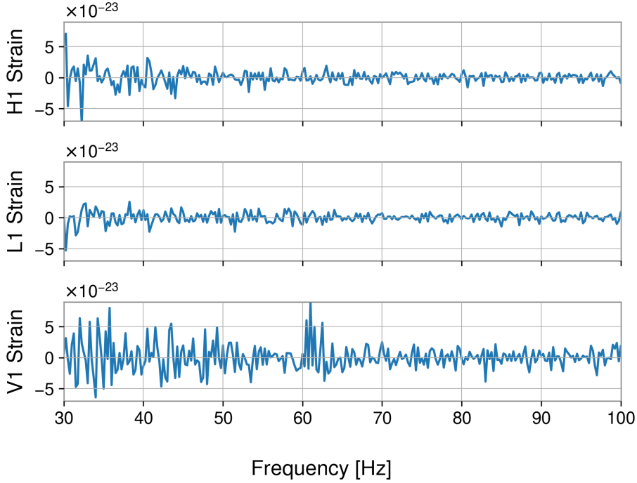
Figure 18. The residual power remaining, from top-to-bottom, in LIGO Hanford, LIGO Livingston, and Virgo when subtracting the best fit non-lensed waveform template for GW200208 as determined by the unlensed PE from the detector strain, over a subset of the total frequency range. As can be seen, there is no obviously coherent oscillatory behaviour in the residual power which would be expected in the case of the microlensing hypothesis. This absence would suggest that what remains is noise related rather than signal related.
