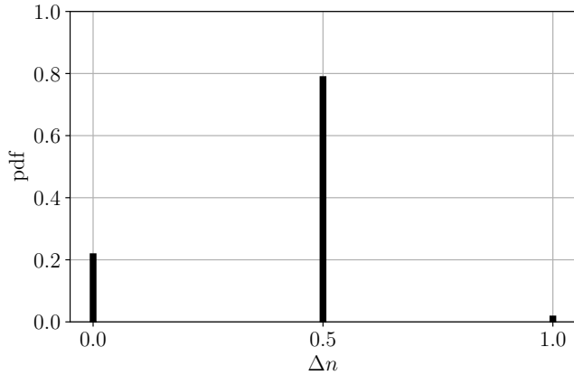
Figure 11. The difference in Morse factor for the GW191230–LGW200104 event pair according to the GOLUM pipeline. The preferred value is 0.5 but there is also some support for 0.
