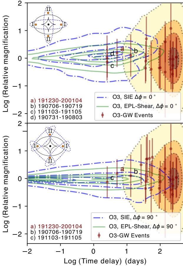
Figure 6. Comparison of the posterior for the observed relative magnification and time delays for the O3 event pairs with the expected distributions for the lensed population of mergers from More & More (2022) (dashed blue, using an SIE model) and from Wierda et al. (2021) (solid green, using an elliptical model with a power low density profile and external shear (EPL-Shear)) and unlensed population (yellow-orange-red), both assuming galaxy lenses. Overlaid in brown are the observed values for selected O3 event pairs, and the letters mark the event pairs more compatible with the lensing hypothesis. Written in brown, and denoted with letter a, is a pair made of a supra-threshold and a sub-threshold event, and further analysed in this work. The top panel corresponds to the expected distribution when the two images are of the same type, i.e., there is no phase difference between the two images (see top-left illustration), while the bottom panel corresponds to a configuration where the two image types differ, i.e., there is a \pi/2 shift between the images. Most of the observed event pairs are well outside the lensed distribution. The GW191103–GW191105, GW190706–GW190719, and GW101230–GW200104 pairs are more compatible with the lensed hypothesis than with the unlensed one. In particular, the GW191103–GW191105 pair lies in a higher probability density region than the other pairs. One also sees that the GW191230–GW200104 pair—made of a supra and a sub-threshold event—lies in a higher density region, even if it is less important than the GW191103–GW191105 pair. This pair is discussed further in Sec. 5.
