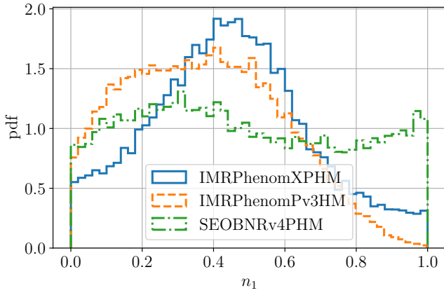
Figure 2. Recovery of the Morse factor for the GW190412 event with different waveforms: IMRPhenomXPHM, IMRPhenomPv3HM, and SEOBNRv4PHM. The support for a type II image is present for the two waveforms from the Phenom family. However, the feature is less prominent for the IMRPhenomPv3HM waveform, and only marginally present for the SEOBNRv4PHM waveform. Therefore, the observed feature is probably spurious and the event is not a type II image.
