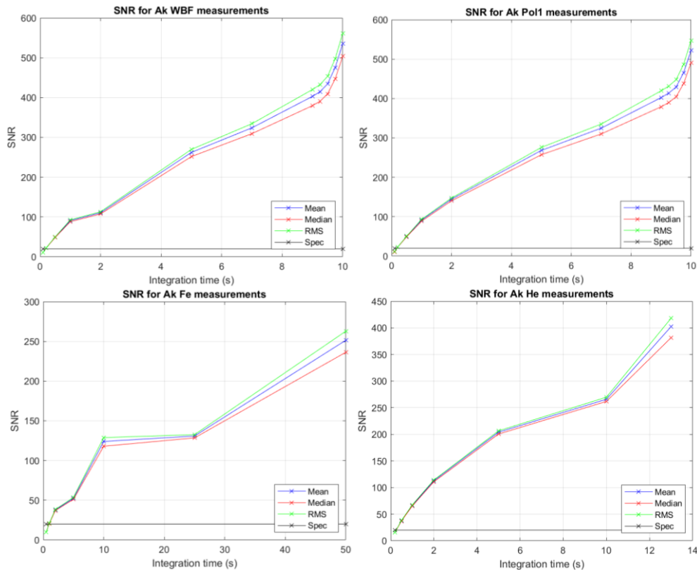
Figure 24: SNR assessment for 4 channels of ASPICCS
