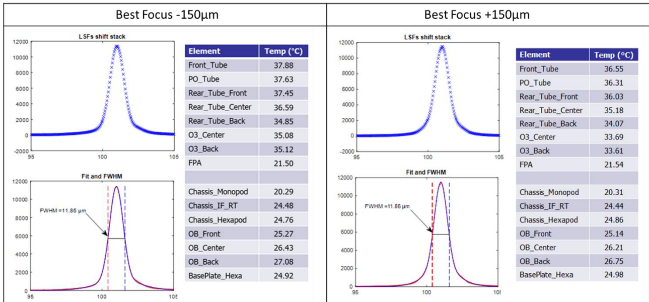
Figure 16: Through focus PSF verification
