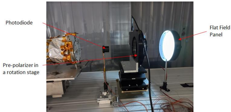
Figure 22. Setup configuration for polarization calibration
