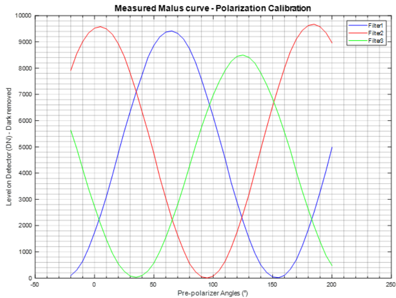
Figure 25. Experimental malus curve retrieval (3 polarizers)
