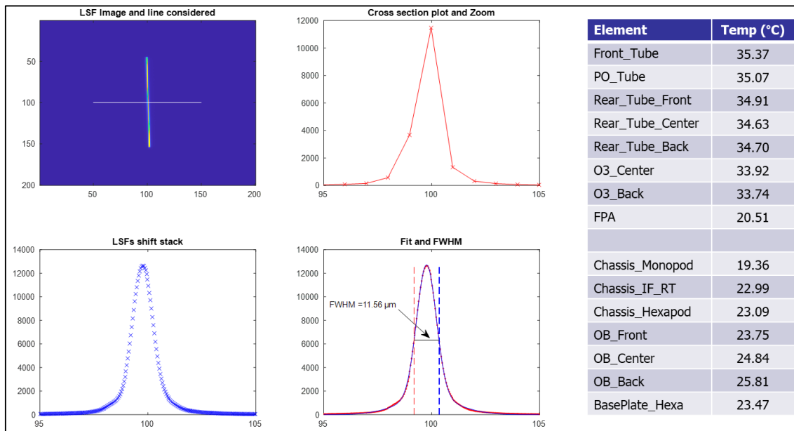
Figure 15. PSF performance at best focus - Operational conditions
