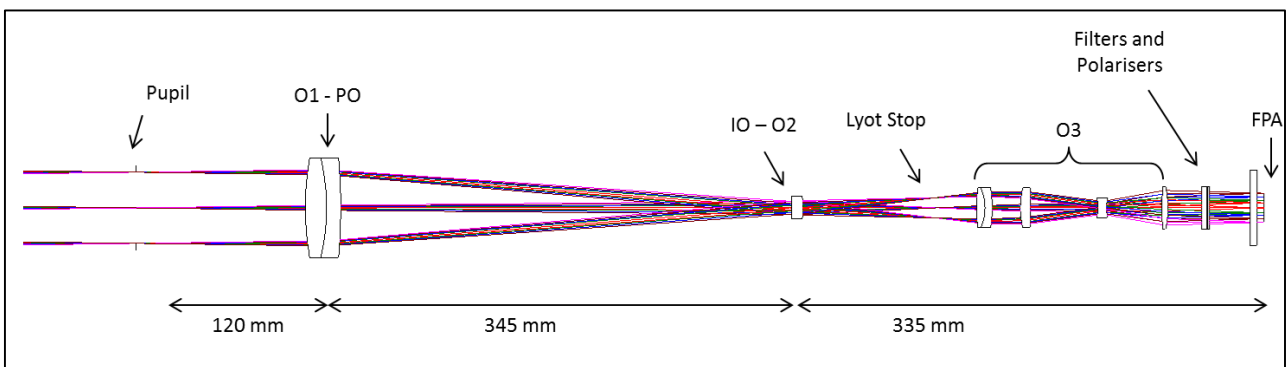
Figure 2. Optical design model of ASPIICS
