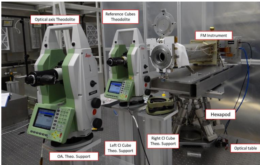
Figure 18: Instrument misalignment measurement setup
