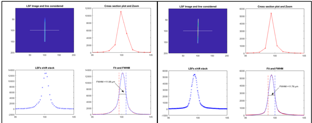
Figure 8. PSF in air, at best focus on hexapod (left) and with ambient shim mounted (right)
