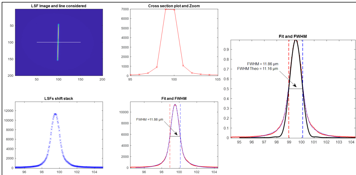
Figure 13. PSF performances at best focus, in air
