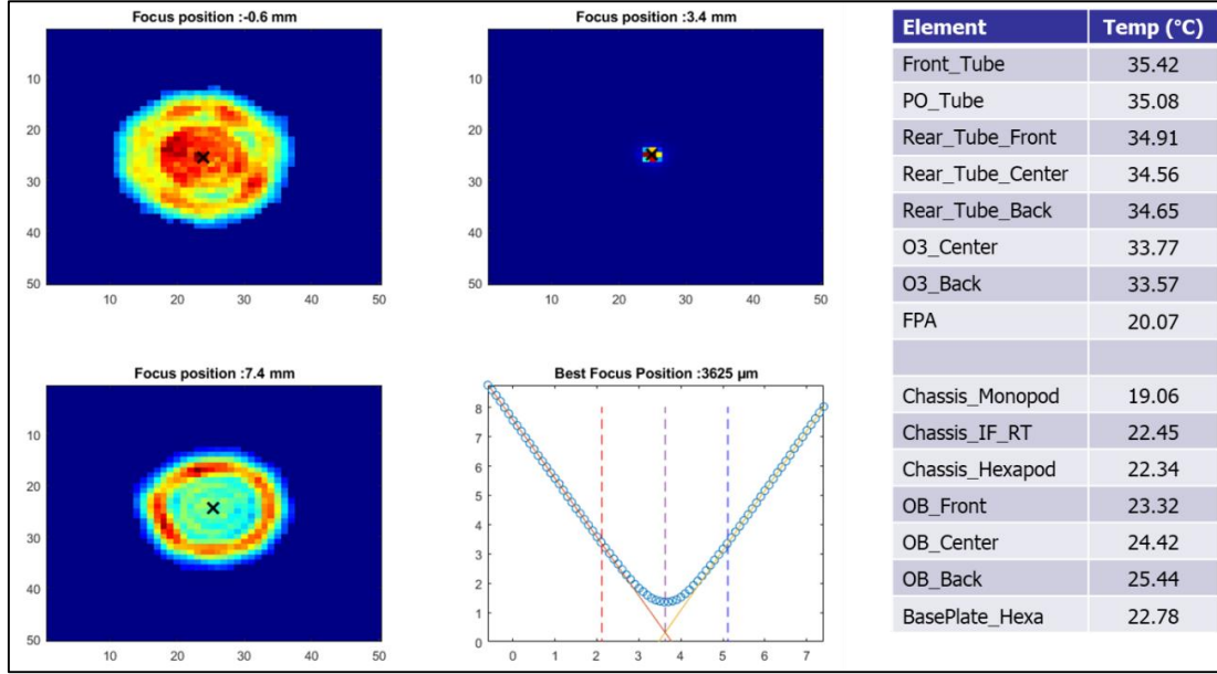
Figure 14. Best focus search results - Operational conditions
