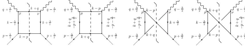
Figure 1. The simplest diagrams contributing to the imaginary part of the amplitude for the scattering \gamma^*\pi \rightarrow \gamma^*\pi . Dashed lines represent the discontinuity of the amplitudes, i.e. their imaginary parts.
