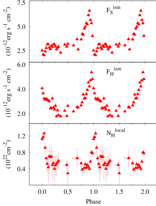
Figure 3: Variation of X-ray flux in soft ( F_S^{ism} ) and hard ( F_H^{ism} ) energy bands along with local hydrogen column density ( N_H^{local} ) estimated from spectral fitting of Swift-XRT spectra of WR 25 in 0.3–10.0 keV energy band. The zero phase corresponds to the time of periastron passage.
