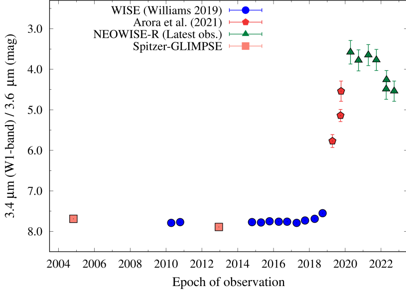
Figure 4: MIR light curve of WR 125 created by combining WISE 3.4 \mu\text{m} (W1-band) data and Spitzer GLIMPSE magnitudes in the 3.6 \mu\text{m} wave band from the literature and the present study.
