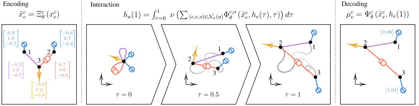
Fig. 4. Neural network architecture. The feature vectors of all hyper-edges are embedded into a latent space using class-specific encoders \Xi_c^c . All addresses are associated with latent coordinates initialized at zero, and then follow a trajectory defined by a differential system whose second member involves couplings born by hyper-edges and defined by neural networks. Addresses interact until \tau = 1 . Finally, hyper-edges exploit the final locations of their addresses to produce a meaningful prediction thanks to class-specific decoders \Psi_e^c .
