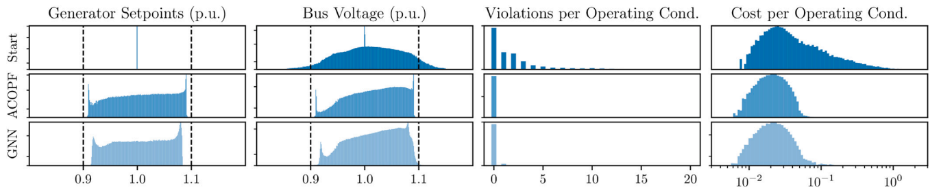
Fig. 7. Comparison of the data distribution before any modification (top row), after the application of the ACOFF solver baseline (middle row), and after the application of our policy trained on the Standard train set (bottom row). All data are from the Standard test set. The first column displays the histogram of all voltage setpoints (control variables) over all generators and all operating conditions. The second column shows the histogram of resulting bus voltage magnitudes over all buses and all operating conditions. The third column contains histograms of the violation count (current or voltage) per operating conditions. The fourth column presents histograms of costs for all operating conditions. The vertical axis is represented in symlog scale (i.e. y \mapsto \ln(y+1) ). Both our trained policy and the ACOFF solver baseline manage to bring the distribution of voltages mostly within authorized bounds ( \underline{V} = 0.9 p.u. and \bar{V} = 1.1 p.u.), although some marginal violations remain.
