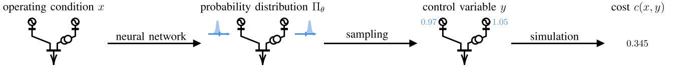
Fig. 1. A power grid operating condition x is passed to a neural network which produces a probability distribution \Pi_\theta(\cdot|x) for each control variable (i.e. generator voltage setpoints). A value for y can thus be sampled, and passed to the cost function c for evaluation, which involves a simulation.
