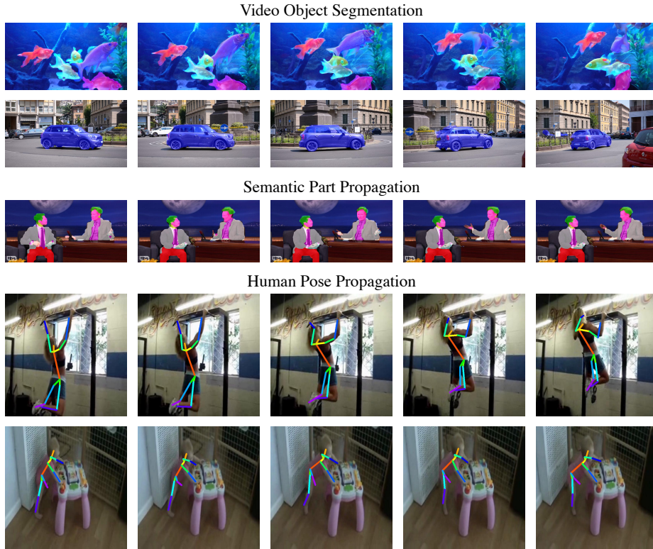
Fig. 4: Qualitative results. We train CropMAE with a ViT-S/16 and qualitatively validate our results on three propagation downstream tasks: video object segmentation (DAVIS-2017 [39]), semantic part propagation [56], and human pose propagation (JHMDB [30]).
