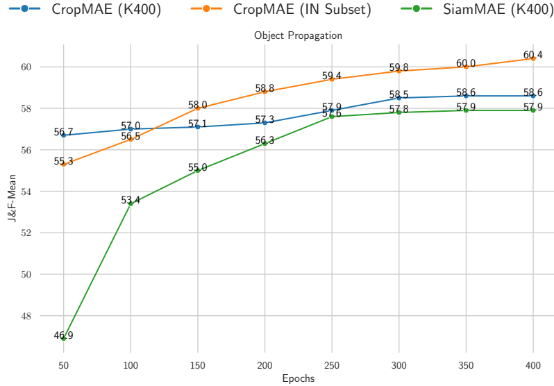
Fig. 6: Performances of CropMAE and SiamMAE on DAVIS during pre-training. For a fixed number of 400 epochs, CropMAE trains faster and yields better results than SiamMAE [23], when trained on K400 frames or ImageNet Subset images.
