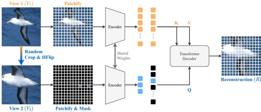
Fig. 1: CropMAE self-supervised learning pre-training. Given an input image ( V_1 ), a second image is generated by performing a random crop and, optionally, a horizontal flip on the original image ( V_2 ). We then patchify [14] both views and mask [25,33] an extremely high portion of the second image (above 98.5%). Both views are encoded by a Siamese [5] ViT encoder, with added positional embedding [14]. A transformer [20] decoder reconstructs the masked image R using self-attention layers on the tokens of the masked image and cross-attention layers between the tokens of the masked and unmasked images.
