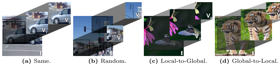
Fig. 2: Illustration of our four cropping strategies. For a given input image I , we generate an unmasked view V_1 and a masked view V_2 following one of four different cropping strategies: (a) Same Views, where V_1 = V_2 ; (b) Random Views, where V_1 and V_2 are two independent random crops; (c) Local-to-Global, where V_1 is a random crop within V_2 , and (d) Global-to-Local, where V_2 is a random crop within V_1 .
