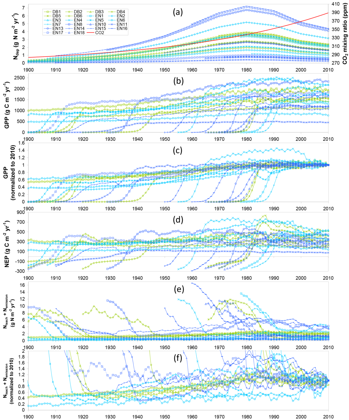
Figure 1. Time courses for 22 forest study sites (DB: deciduous broadleaf; EN: evergreen needleleaf) of (a) assumed atmospheric N_r deposition ( N_{dep} ) and CO_2 mixing ratio; and baseline model simulations of (b) gross primary productivity (GPP), (c) GPP normalized to the 2010 value, (d) net ecosystem productivity (NEP), (e) total N losses by leaching ( N_{leach} ) and gaseous emissions ( N_{emission} ), and (f) total N losses normalized to 2010.
