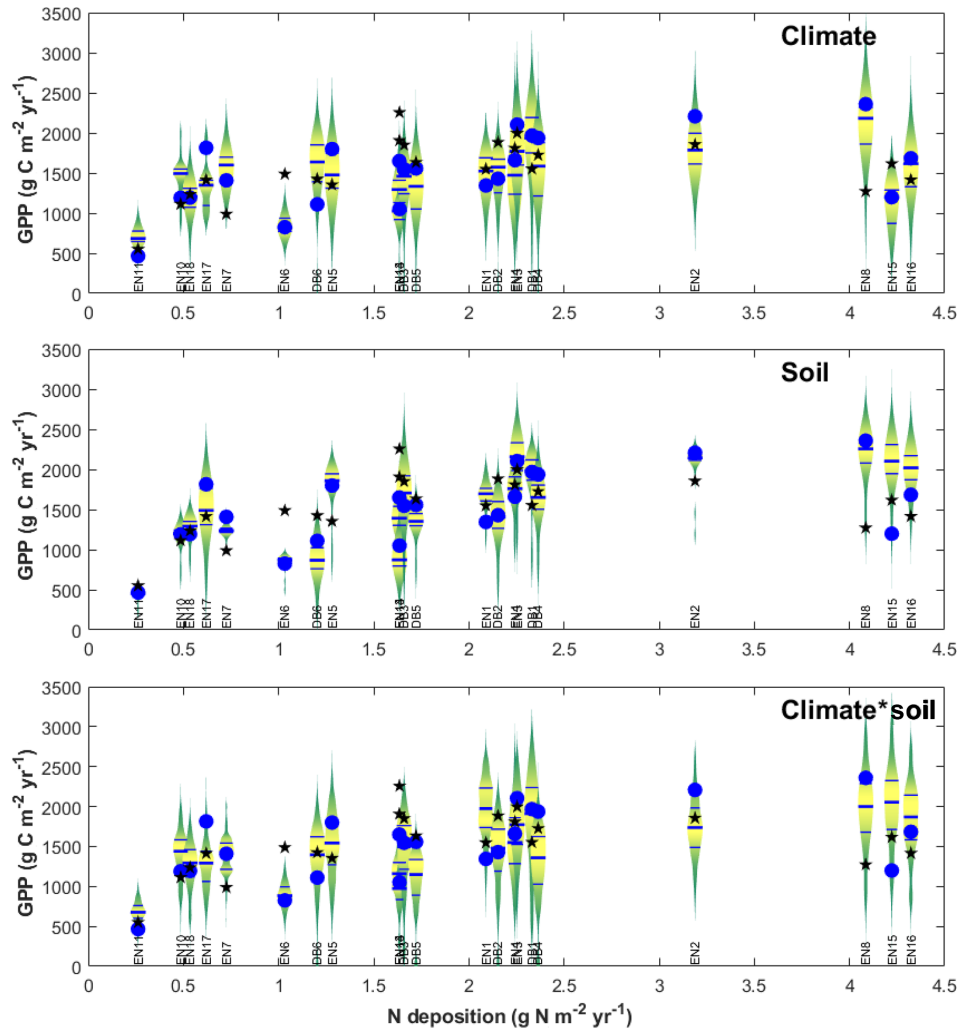
Figure 6. Input sensitivity study for gross primary productivity (GPP) modelled at each forest monitoring site for different soil/climate scenarios (vertical violin plots), compared with model base runs GPP_{\text{base}} (blue circles) and EC-derived GPP_{\text{obs}} (black stars). The data are displayed as a function of N_{\text{r}} deposition over the CEIP–NEU measurement periods, for n = 22 deciduous broadleaf (DB) and coniferous evergreen needleleaf (EN) forest ecosystems. For each site, the violin plot shows the range and distribution (median, quartiles) of GPP modelled at the site using climate and/or soil input data from all 22 sites, showing the sensitivity to model inputs other than N deposition. See text for details.
