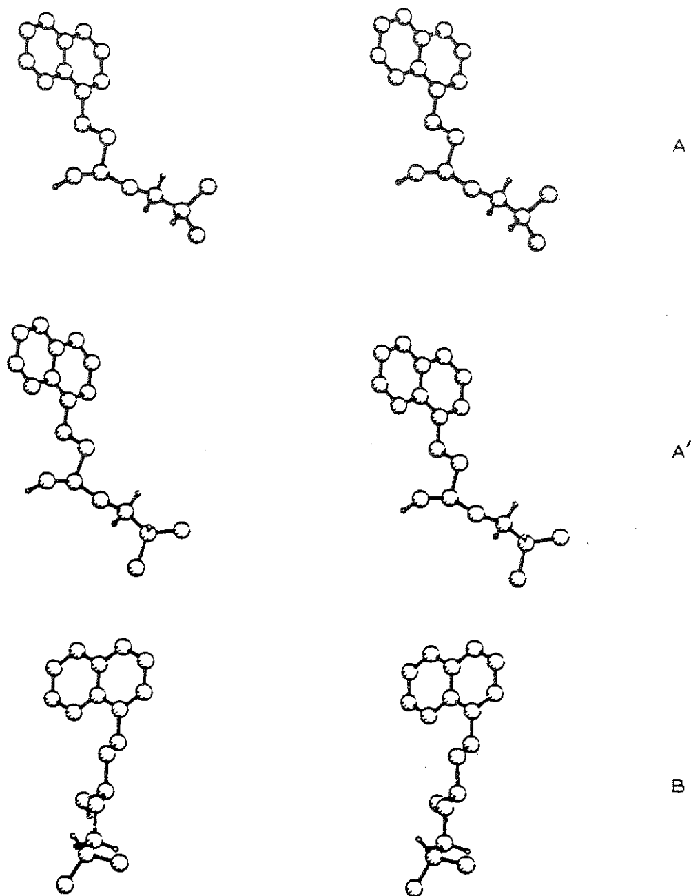
Fig. 3. Stereoscopic views of the most probable conformer for propranolol.
