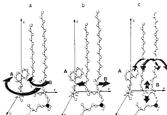
Fig. 2. Schematic presentation of the packing procedure used to assemble molecules in mixed monolayer.
