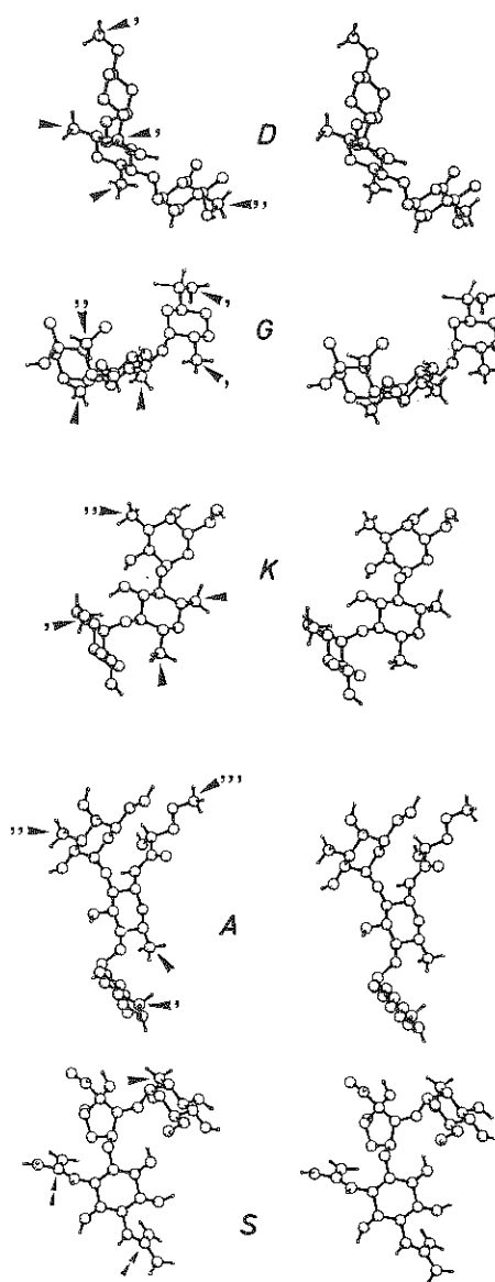
Fig. 5. Stereoviews of the most probable conformer of aminoglycosides after minimization procedure (D dibekacin; G gentamicin; K kanamycin; A amikacin; S streptomycin). The arrowheads point to the ionized atom of each amino (or guanido) function. For orientation of gentamicin, dibekacin, kanamycin A and amikacin the amino groups situated on the aminohexose linked in position 4 of the deoxystreptamine (i.e. on the right in Fig. 4) are denoted '1' whereas those on the 6-linked aminohexose are denoted '2'; for streptomycin the guanidium groups are indicated by a double arrow. The component of gentamicin shown is the Cla (see legend of Fig. 4); no important difference was observed between gentamicin C 1 , C 1a and C 2 . The conformer of tobramycin is very similar to that of dibekacin.
