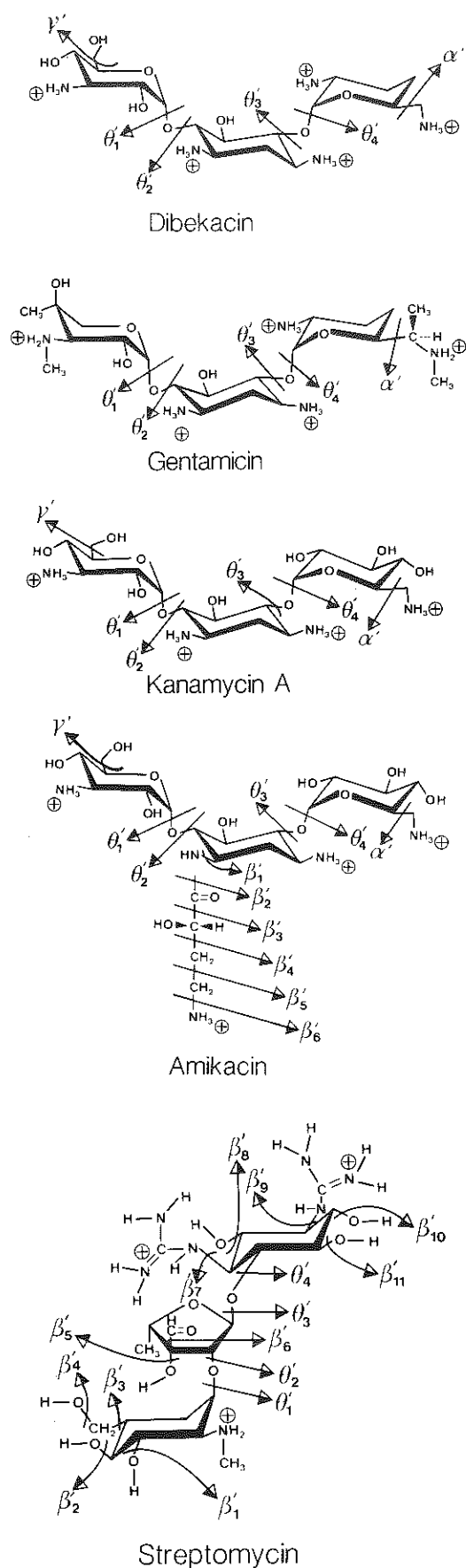
Fig. 4. Structural formulae of the aminoglycosides studied and definition of the torsional angles. The structural formulae used are those given in refs. 44–47. The component of gentamicin shown is the C1 (C1a 6'-dihydro-6'-amino; C2 6'-methyl-6'-amino). Tobramycin is 4'-hydroxy-dibekacin.
