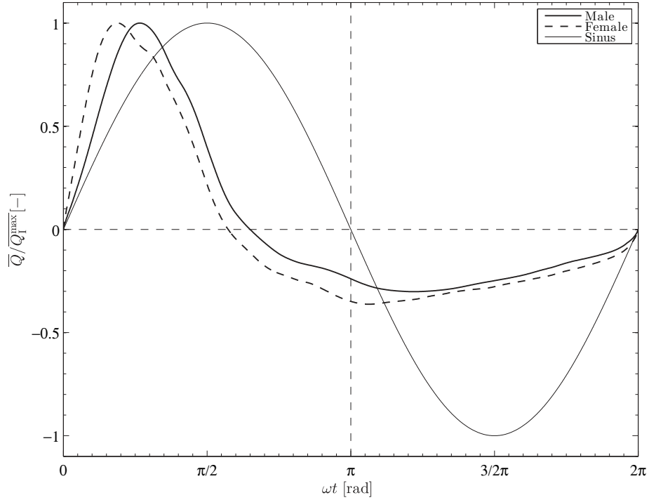
Fig. 3. Normalized mean flow rates \bar{Q}/\bar{Q}_{\max}^{\max} as function of \omega t [rad] for the specific inhalation task Aerosol and males and females.
