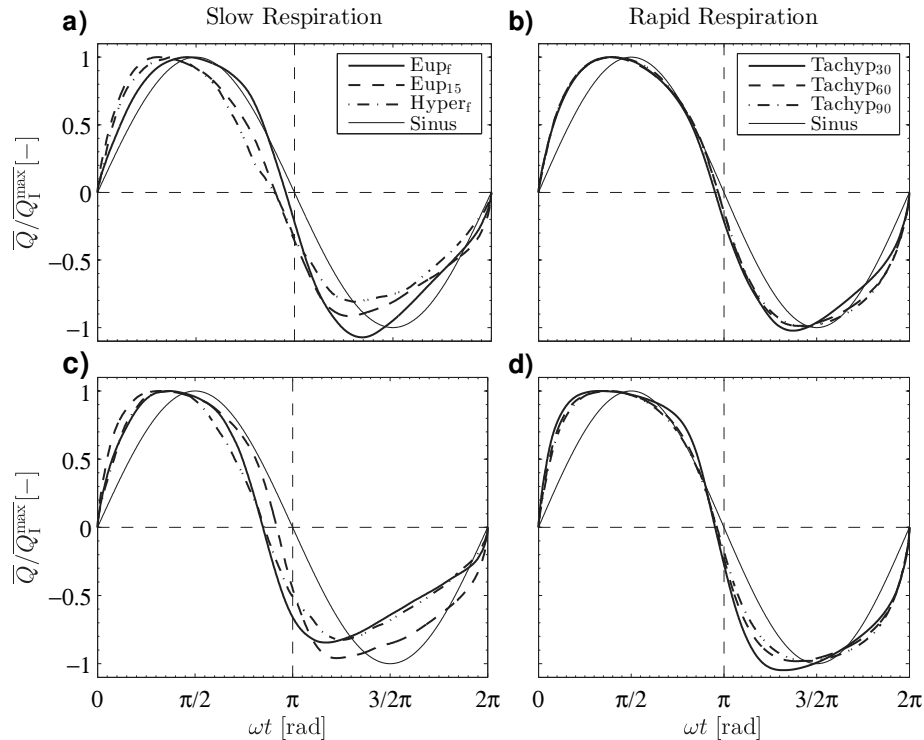
Fig. 2. Normalized mean flow rates \bar{Q}/\bar{Q}_I^{\max} as function of \omega t [rad] for slow breathing tasks ( Eup f , Eup 15 , Hyper f ) (Panels a and c for males and females, respectively) and rapid breathing tasks ( Tachyp 30 , Tachyp 60 , Tachyp 90 ) (Panels b and d for males and females, respectively).
