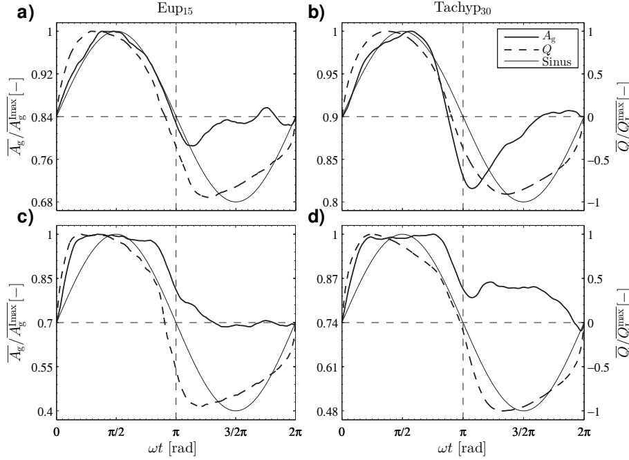
Fig. 6. Comparison of mean, normalized glottal area \bar{A}_g/\bar{A}_g^{\max} , mean, normalized flow rate \bar{Q}/\bar{Q}_i^{\max} , and sinusoidal pattern for males (panels a and b, tasks Eup 15 and Tachyp 30 , respectively) and for females (panels c and d, tasks Eup 15 and Tachyp 30 , respectively). Results are given for the subjects with “dynamic” glottal variations (2nd group).
