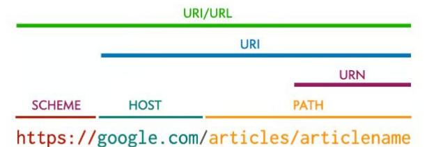
URL Structures
