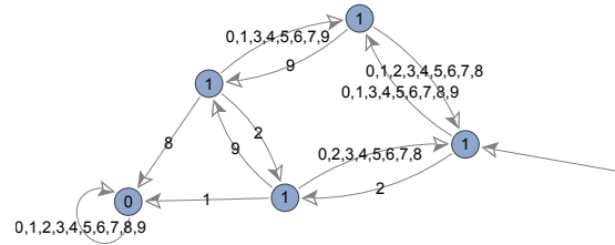
Fig. 1. The sequence (s_n)_{n \geq 0} is generated by the base-10 DFAO (it reads base-10 representations with least significant digit first)
