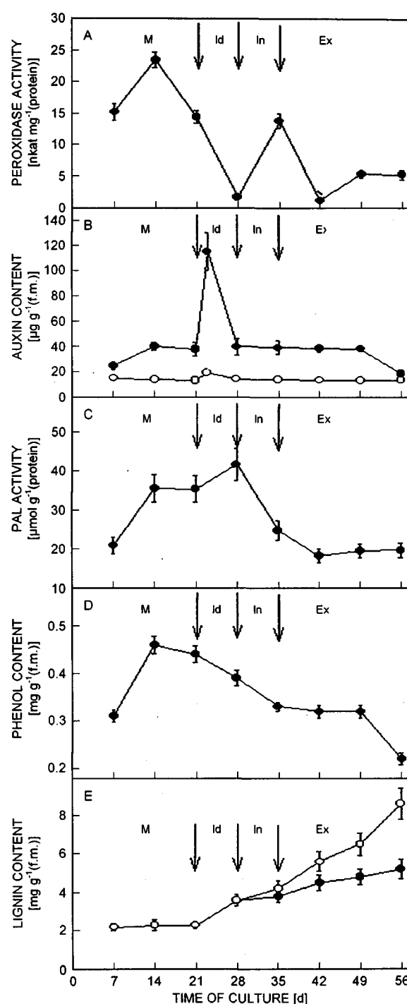
Fig. 1. Rooting process of walnut shoots: A - soluble peroxidase activity; B - contents in free IAA (closed circles) and conjugated IAA aspartate (open circles); C - phenylalanine ammonia-lyase activity; D - phenol content; E - lignin content of micropropagated walnut shoots with (open circles) or without (closed circles) root emergence during the rooting expression phase. Means ± SE, n = 3; M - preceding multiplication phase, Id, In, Ex - rooting induction, initiation, and expression phases, respectively.
