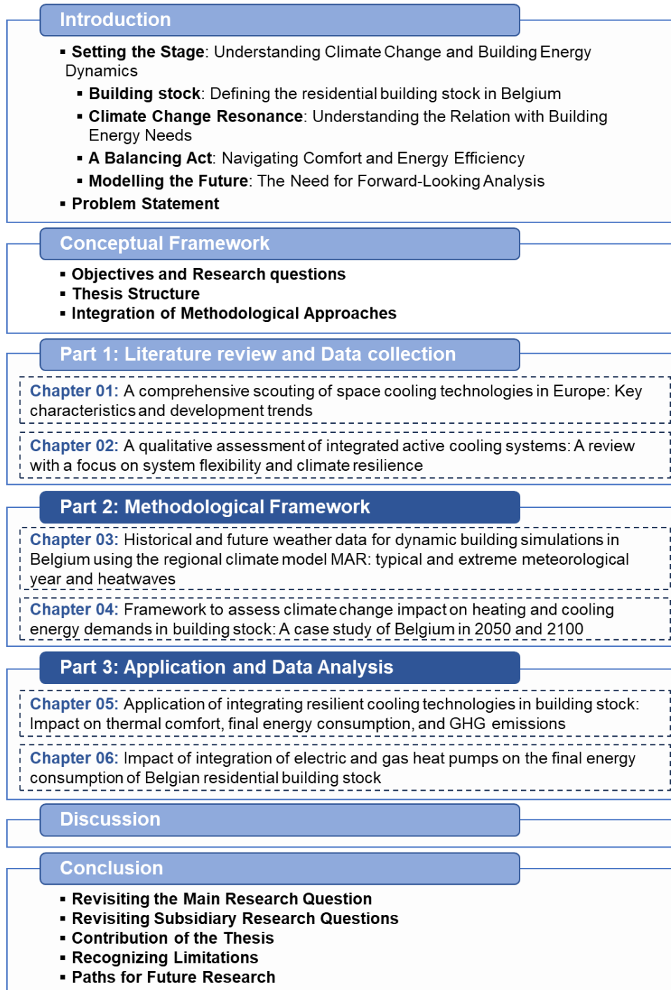
Figure 2.1. Thesis structure
