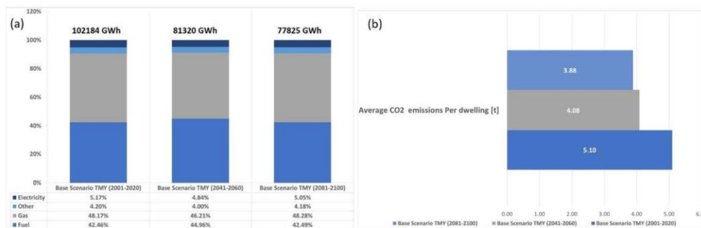
Fig. 6 - Comparison between the SH and DHW energy consumption in the Base Scenario in different years (a) Total SH and DHW energy consumption (b) average CO 2 emissions per dwelling.
