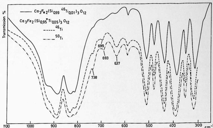
Fig. 2. Typical infrared spectra of synthetic titanium andradites
