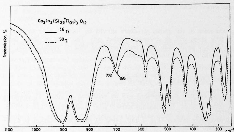
Fig. 1. Typical infrared spectra of synthetic titanium indium garnets
