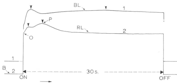
Fig. 2. Time course of the fluorescence emission at 685 nm measured at room temperature of a flashed leaf (500 flashes) pre-illuminated for 30 sec with intense blue light (BL) and of a flashed leaf (900 flashes) pre-illuminated for 60 sec with intense red light (RL). The leaves were kept in darkness for 60 sec between the end of the pre-illumination and the registration of the time course of the fluorescence emission.
