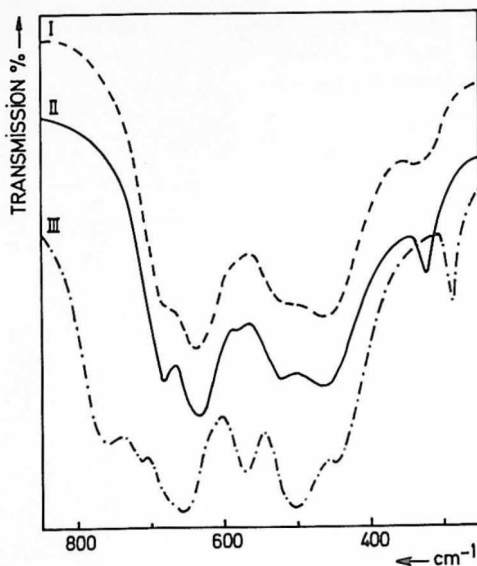
FIG. 1. Infrared spectra of cubic Zn_4AlSbO_8 (I, disordered; II, ordered) and of orthorhombic Mg_4AlSbO_8 (III). For the latter compound, bands in the 800\text{--}700\text{ cm}^{-1} region point to the existence of AlO_4 tetrahedra; these bands are missing in the spectra of Zn_4AlSbO_8 , where all Al^{3+} cations should be octahedrally coordinated.
