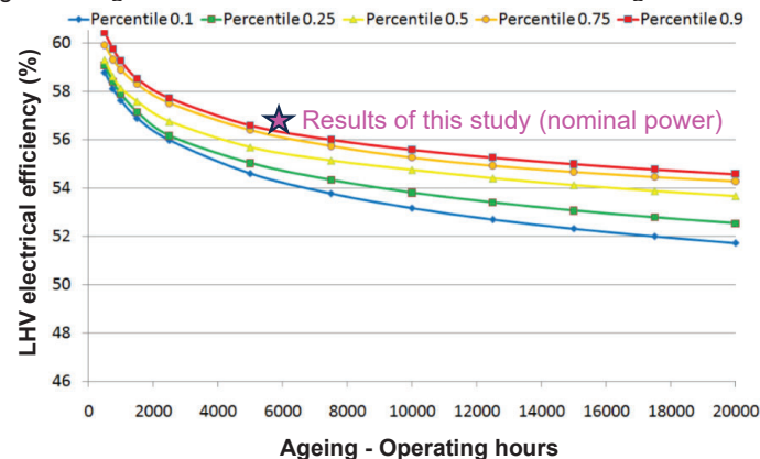
Figure 10. Statistical analysis of production systems back in 2011 [19] expressed in terms of LHV electrical efficiency decay over time at nominal output power (1500 W el ). System's version in the results published by the manufacturer has not been disclosed. Reproduced from reference with the addition of this study's laboratory results.
