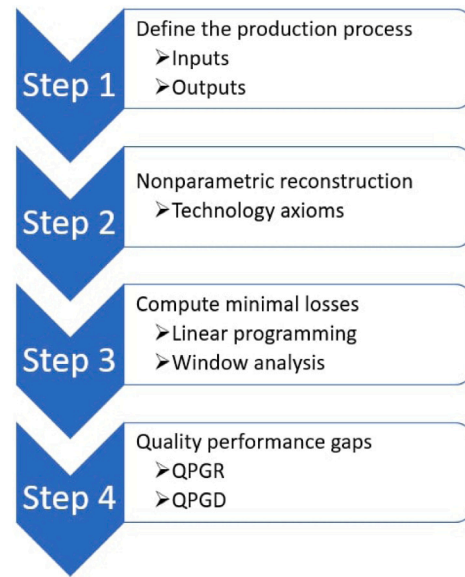
Fig. 1. Empirical strategy.
