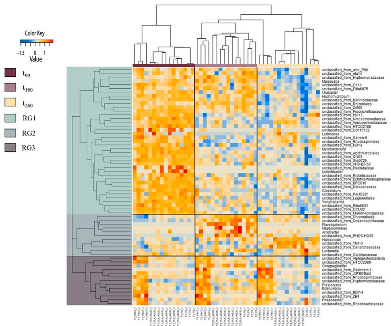
Fig. 5. Heatmap of the 63 genera significantly affected by the polymer chemical composition, (polylactic acid (PLA), polybutylene adipate-co-terephthalate (PBAT), polystyrene (PS)) and by the immersion time (99 days ( t_{99} ); 160 days ( t_{160} ) and 260 days ( t_{260} )). Three response groups (RGs) were defined with hierarchical clustering based on center-scaling abundance.
