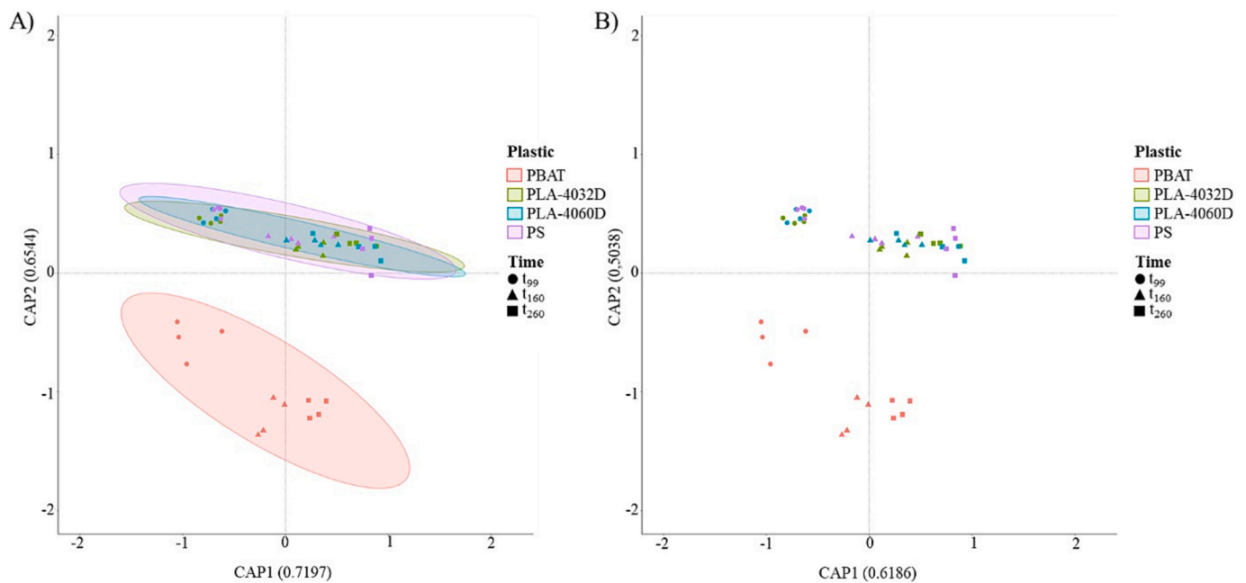
Fig. 3. (A) Constrained analysis of principal coordinates (CAP) scaling analysis profile of the pairwise community dissimilarity (Bray-Curtis) index of the 16S sequencing data of plastics after 99 days ( t_{99} ), 160 days ( t_{160} ), and 260 days ( t_{260} ) of immersion in the marine aquarium; (B) CAP scale analysis using a variance adjusted weighted UniFrac (polylactic acid (PLA), polybutylene adipate-co-terephthalate (PBAT), polystyrene (PS)). ANOVA with 1000 permutations indicated that the plastic chemical composition and the immersion time significantly influenced the bacterial communities ( p -value = 0.000999 and 0.000999, respectively).
