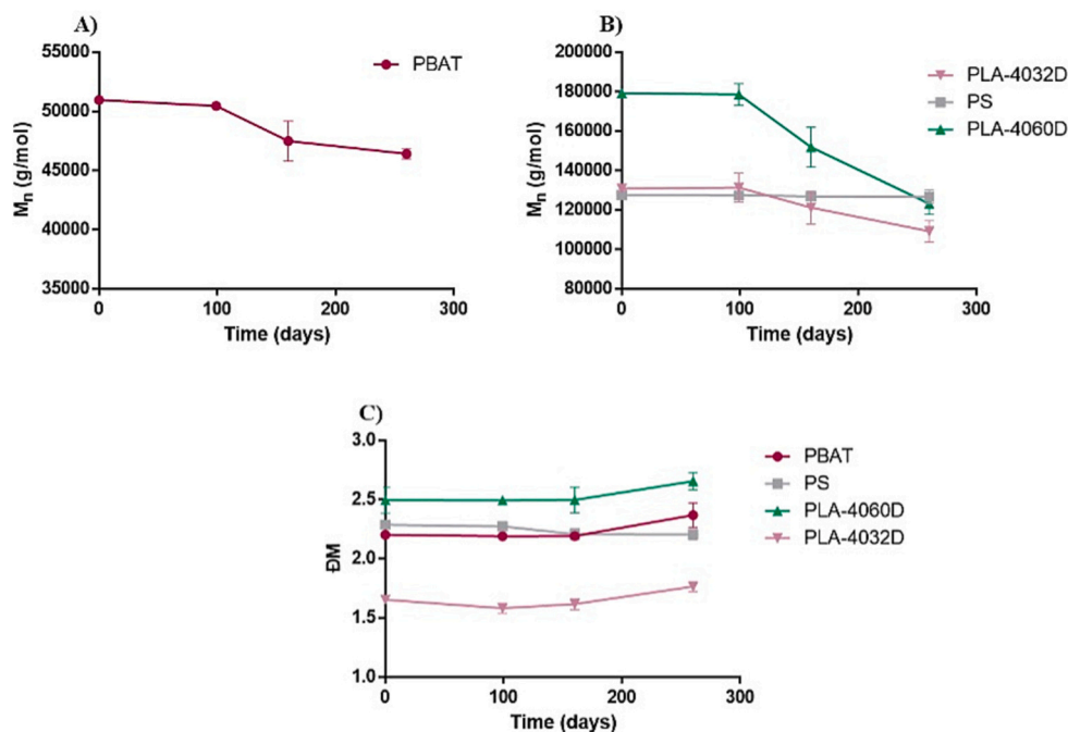
Fig. 2. Number average molecular weight ( M_n ) (A & B) and dispersity ( \overline{M}_w/\overline{M}_n ) evolution (C) of the plastic films (semicrystalline PLA (4032D); amorphous PLA (4060D); PBAT and PS) before and after the different immersion times (99, 160 and 260 days) in the marine aquarium (polylactic acid (PLA), polybutylene adipate-co-terephthalate (PBAT), polystyrene (PS)).
