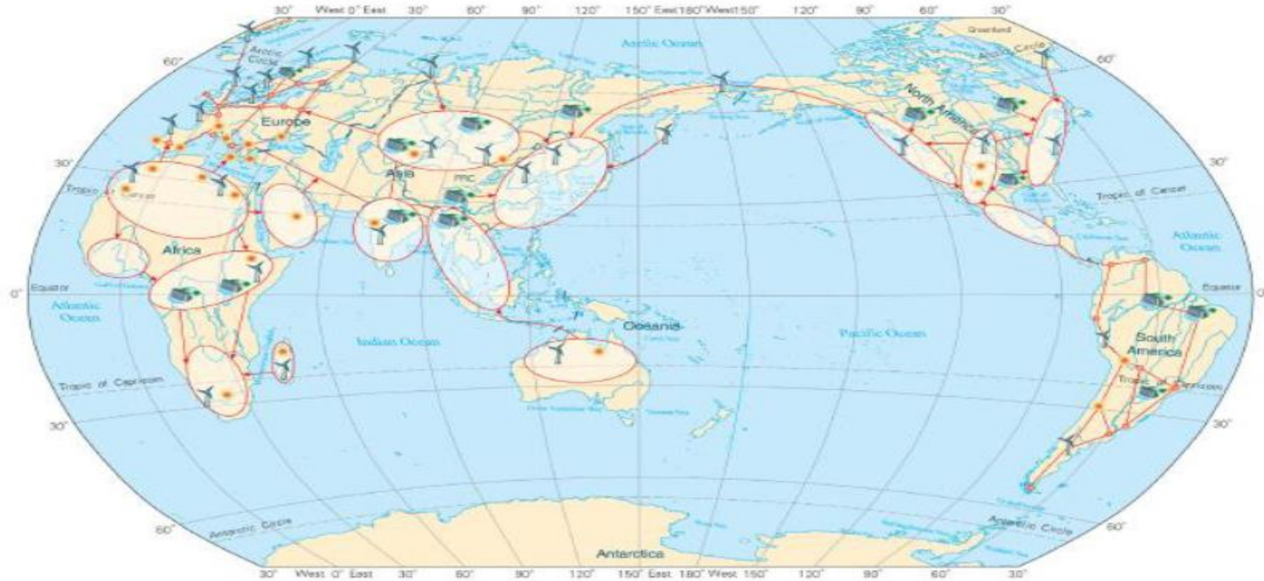
Figure 2-3. Schematic representation of the backbone electricity interconnection [13]
