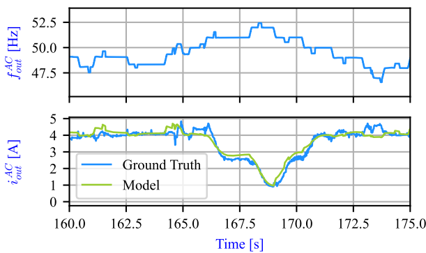
Figure 2: Comparison between PV inverter model ( \hat{F}(z) ) and measurements for different values of f_{out}^{AC} .
