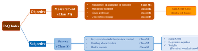
Fig. 8. Scoping/Mapping diagram of IAQ indexes.
