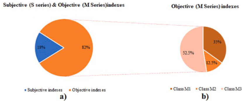
Fig. 7. a) Distribution of IAQ indexes reviewed in this study based on survey/measurement (subjective/objective) classification, and b) the distribution of M series indexes.
