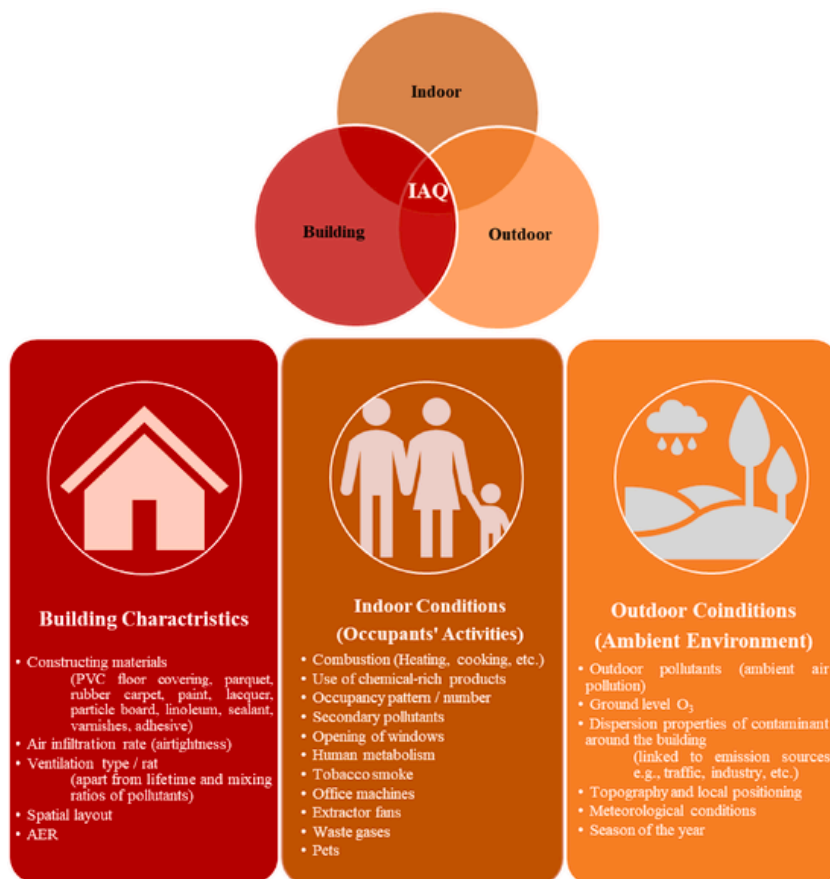
Fig. 1. Main IAQ determinants with examples.
