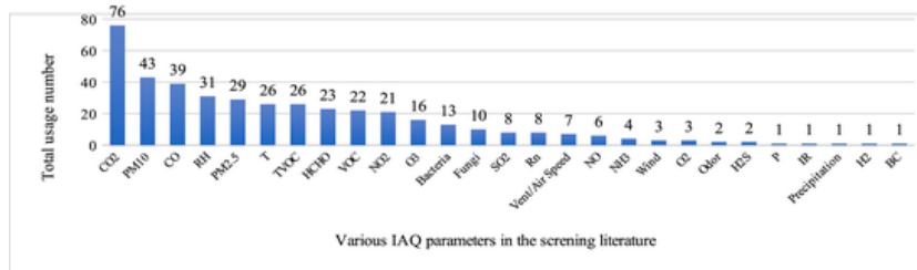
Fig. 6. Distribution of different IAQ indicators among 110 studies in the screening stage of index scoping review. (BC, IR, Rn, TVOC and P, stand for Black-Carbon, Solar irradiance, Radon, Total VOC and Pressure, respectively.)
