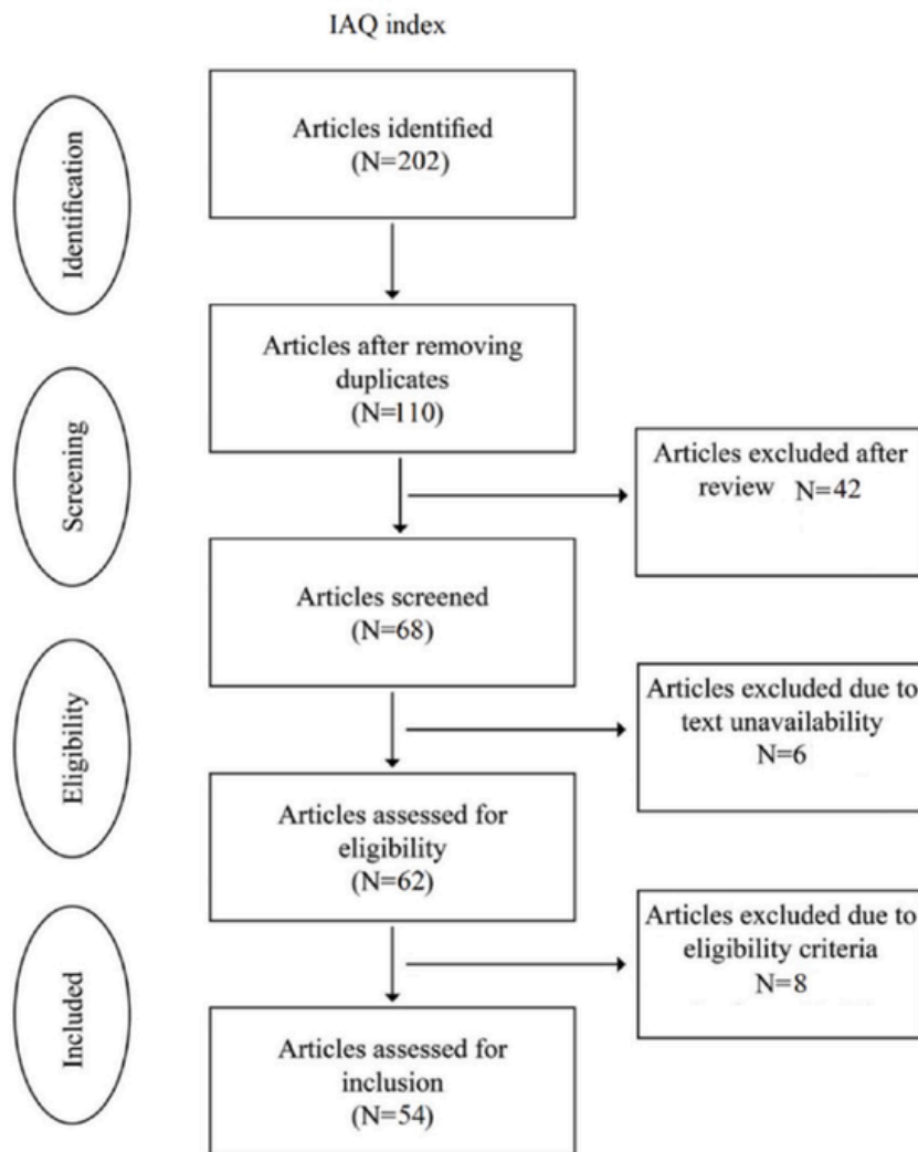
Fig. 3. Schematic diagram and the corresponding statistics of the PRISMA framework.
