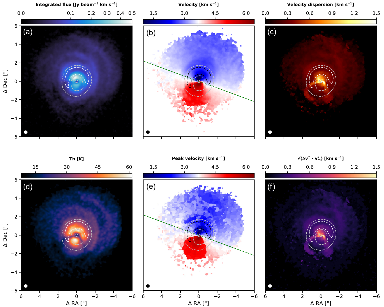
Figure 2. Moment maps. (a)–(f) moment 0, moment 1, moment 2, peak brightness temperature, peak velocity, and velocity dispersion minus thermal component for ^{12}\text{CO} , respectively. All integrated maps, with the exception of peak brightness temperature, are continuum subtracted. The continuum contour at 13.6 \text{ mJy beam}^{-1} ( 0.2 \times maximum) is given in white [in panels (a), (c), (d), (f)] and black [in panels (b) and (e)]. A secondary continuum contour at 1 \text{ mJy beam}^{-1} ( \sim 20\sigma ) is given in silver . The green-dashed lines in panels (b) and (e) represent the rotation axis of the outer disc. Beam is given on the bottom left corner. The features seen towards the SE and SW directions (PAs \approx 110^\circ and 190^\circ ) in panels (c), (d), (e), and (f) are due to the intervening cloud (Casassus et al. 2013b); an attempt at cloud correction is shown in Appendix A along with a description on the procedure.
