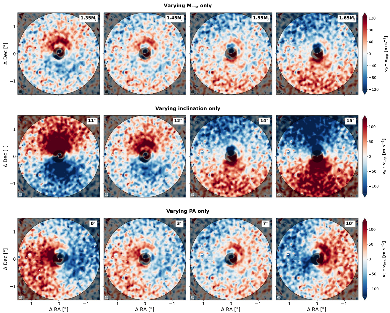
Figure C1. Uncertainty series: ^{12}\text{CO} residual velocity maps for varying quantities of M_{\odot} , inclination and PA around the best-fitting values determined from the MCMC fitting in EDDY.
