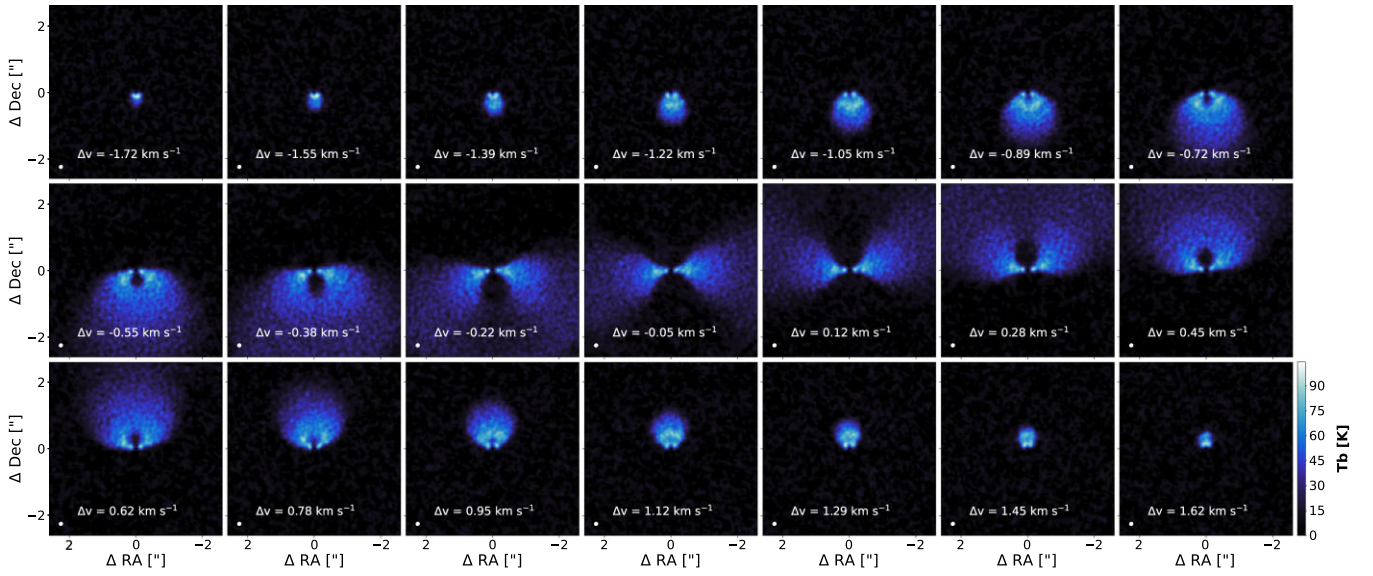
Figure B1. ALMA data: ^{12}\text{CO } J=2-1 channel maps.
