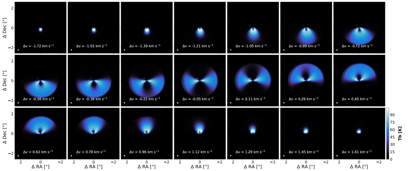
Figure B2. MCFOST synthetic data: ^{12}\text{CO } J=2-1 channel maps with an embedded 10M_J planet at 38 au from disc centre.
