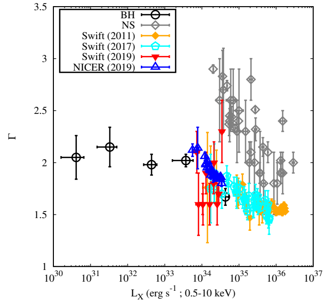
Figure 3. Comparison of the spectral (photon index \Gamma )– X-ray luminosity ( L_X , 0.5–10 keV) behaviour of J1357 (coloured points, see legend, assuming d = 6 kpc) with other low-level accreting LMXBs as compiled by Wijnands et al. (2015) for both BH (solid black points) and NS (grey points) transients. The earlier J1357 values are from Armas Padilla et al. (2013) and Beri et al. (2019a) for the 2011 and 2017 outbursts respectively.
