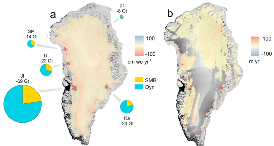
Figure 3. Greenland dynamic mass balance, 2011–2014. (a) Difference between Cryosat-2 and RACMO2.3 mass balance. (b) Ice velocity change between 2000–2001 and 2008–2009 mapped by imaging Synthetic Aperture Radar [Joughin et al. , 2010]. Several marine-terminating glaciers exhibiting signs of dynamic ice loss are apparent; Kangerdlugssuaq (Ka), Jacobshavn Isbræ (JI), Upernavik Isstrøm (UI), Steenstrup (SP), and Zachariae Isstrøm (ZI); all of which have undergone velocity change during the preceding decade. For each of these glaciers, the total 4 year mass loss from the rapidly thinning terminus regions, bounded by the gray lines, is shown. The color wheels indicate the partitioning of mass losses within the bounded regions, according to surface mass and dynamic processes, with the radius of each wheel scaled according to the magnitude of the total losses. The background image is the MODIS mosaic of Greenland [Haran et al. , 2013] overlaid with a shaded relief of ice sheet elevation.
