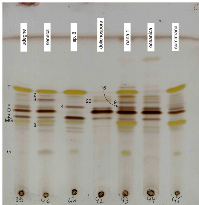
Fig. 18 TLC in phase C for representatives of the polydactyloid clade. See Table S1 for detailed voucher information. D = dolichorrhizin, G = gyrophoric acid, M = methylgyrophorate, P = peltidactylin, T = tenuiorin, Z = zeorin. See Material and Methods for details.
