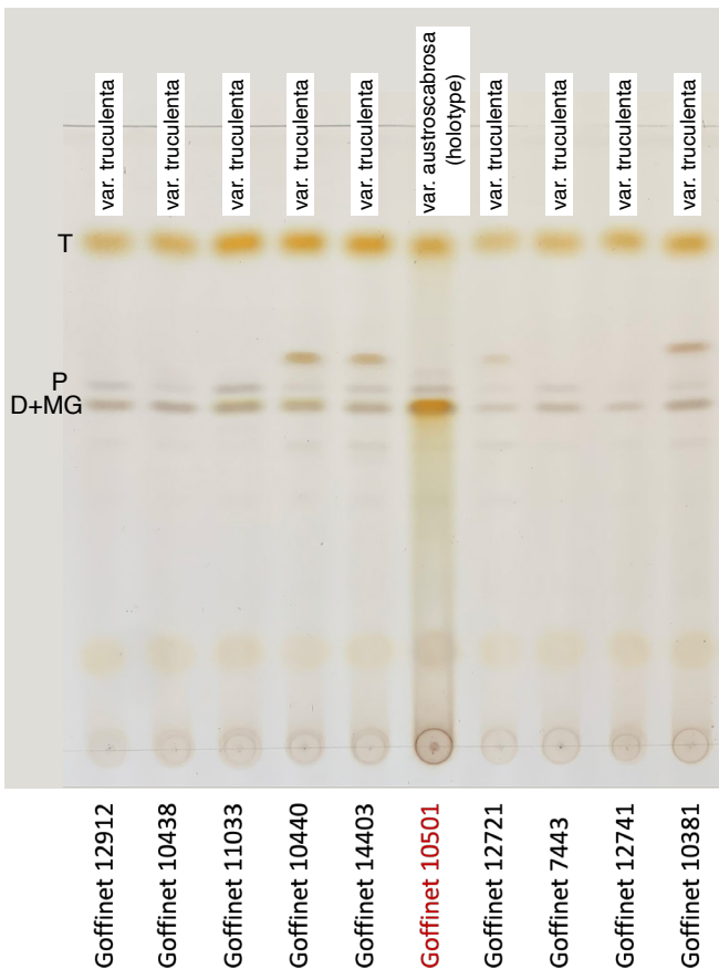
Fig. S3 TLC in phase C for representatives of P. truculenta (incl. var. austroscabrosa ). See Table S2 for detailed voucher information. D = dolichorrhizin, G = gyrophoric acid, M = methylgyrophorate, P = peltidactylin, T = tenuiorin, Z = zeorin. See Material and Methods for details.
