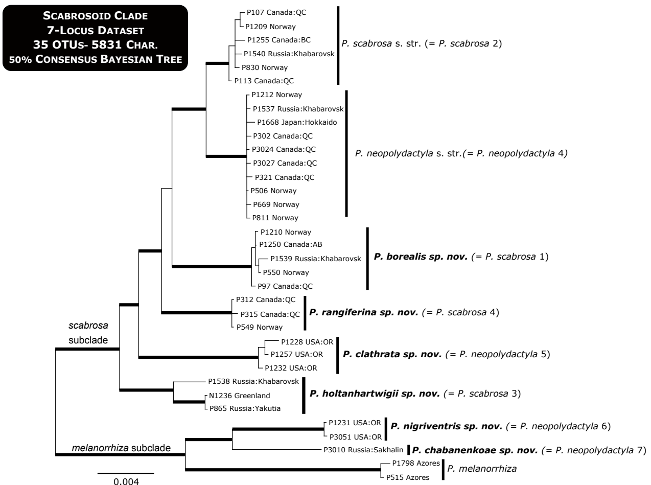
Fig. 3 Phylogenetic relationships within the scabrosoid clade. 50% consensus Bayesian tree modified from Magain et al. (2017b). Thick branches have bootstrap support values equal to or above 70%. Vertical bars indicate delimitations of species as circumscribed in this study. Species newly described are shown in bold . Informal taxon names used in previous studies (Magain et al. 2017a, b) are indicated in parentheses.
