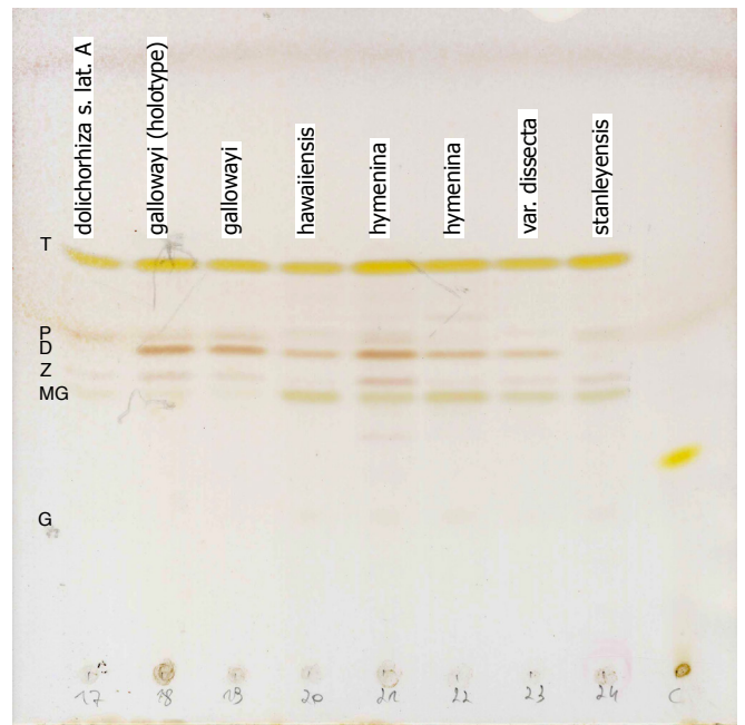
Fig. S4 TLC in phase C for representatives of Peltigera hawaiiensis and P. gallowayi . See Table S2 for detailed voucher information. D = dolichorrhizin, G = gyrophoric acid, M = methylgyrophorate, P = peltidactylin, T = tenuiorin, Z = zeorin. See Material and Methods for details.
