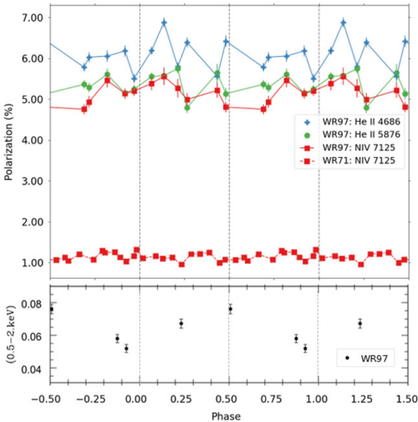
Figure 1. RSS line polarization phase variations for 3 emission lines in WR97 ( top, upper solid lines ), compared with its Chandra X-ray variations in the 0.5–2 keV band ( bottom ). Polarization of one representative line of WR71 is also shown for comparison ( top, lower dashed line ), with error bars smaller than the points.
