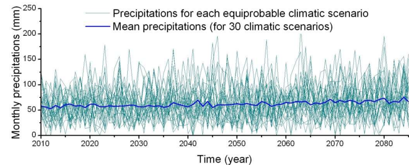
August precipitations
