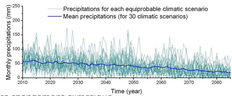
August precipitations
