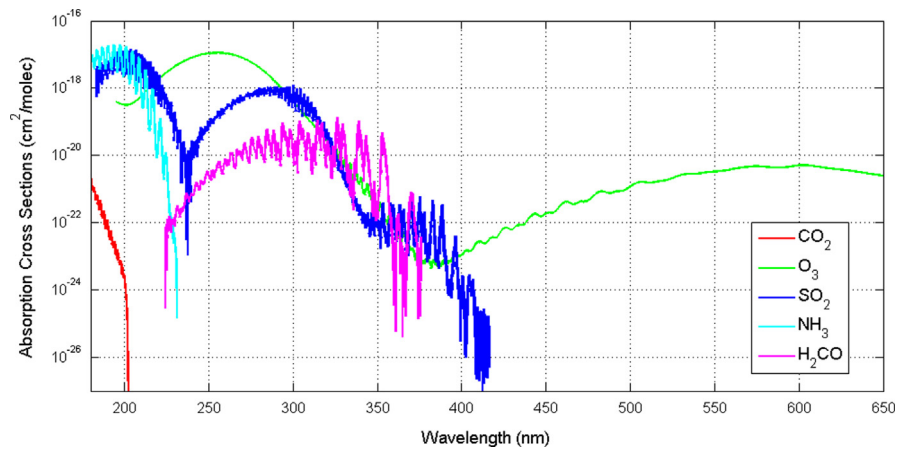
Fig. 1. Absorption cross sections of \text{CO}_2 , \text{H}_2\text{CO} , \text{NH}_3 , \text{SO}_2 , and \text{O}_3 considered in this study.
