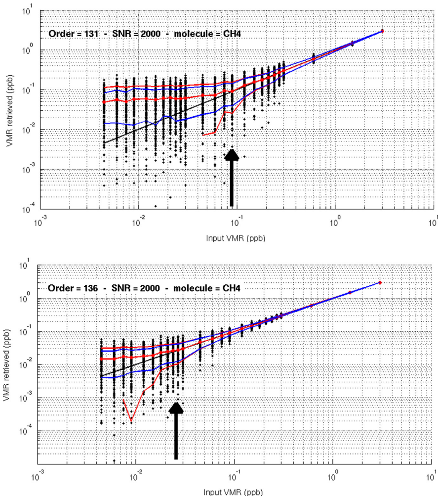
Fig. 3. Example of results in the case of methane: (top) for the order 131 (2944.5–2968.1 cm -1 ) and (bottom) for the order 136 (3056.9–3081.4 cm -1 ). The black dots are the individual (initial-retrieved) abundances of CH 4 ; the red circles are the average retrieved value for each injected abundance; the red curves are the retrieved average \pm the average error on the retrievals; the blue curves are the retrieved averages \pm the standard deviation of the retrieved values and the black line represent the ideal retrieval (=injected value). The arrows indicate the detection limit values when the average error starts to be larger than the standard deviation. (For interpretation of the references to color in this figure legend, the reader is referred to the web version of this article.)
