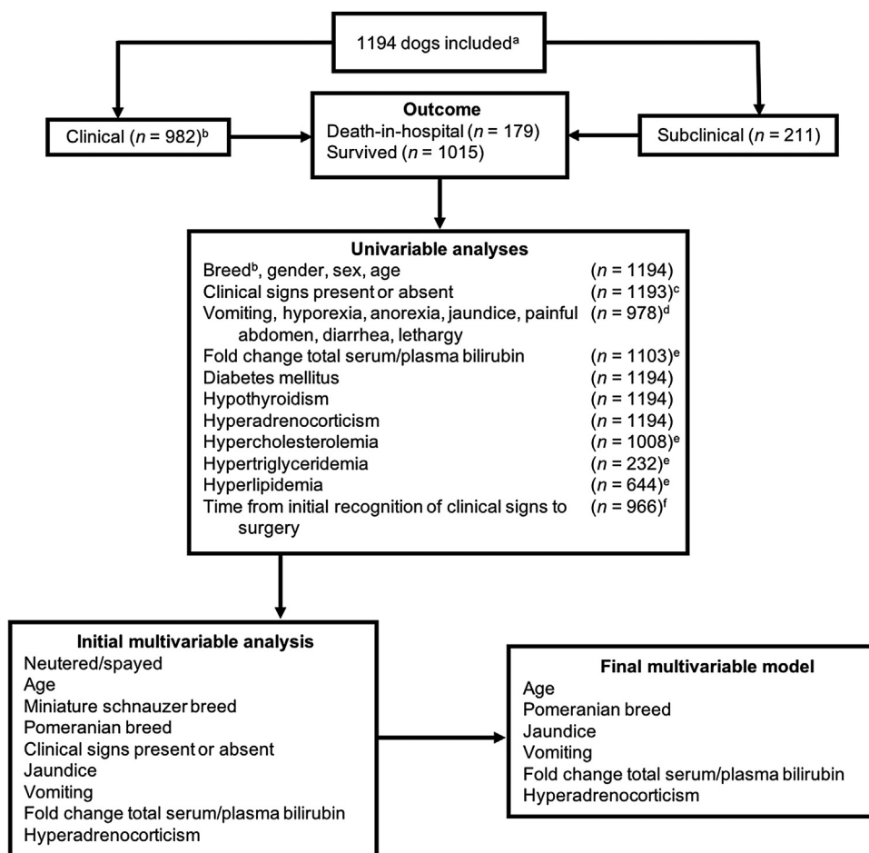
Fig. 1. Flow diagram. A total of 1194 dogs with gallbladder mucocèles were included in the study. a There were no dogs excluded. Several potentially clinically significant variables were included in univariable logistic regression analyses. b The 10 most common breeds were included (i.e. Mixed breed, Shetland sheepdog, Cocker spaniel, Miniature schnauzer, Bichon frise, Pomeranian, Border terrier, and Chihuahua). c One dog did not have a clear distinction if clinical signs were present or absent in the 7-days preceding cholecystectomy. d The seven most commonly reported clinical signs (i.e. vomiting, hyporexia, anorexia, jaundice, painful abdomen, diarrhea, and lethargy). e Biochemical parameters (total serum/plasma bilirubin, cholesterol, and triglyceride concentrations) were performed at the discretion of the attending clinician, which resulted in missing data for these variables. f Time (days) from initial recognition of clinical signs to cholecystectomy was missing in 16/982 clinical dogs. Significant variables in the univariable analyses ( P < 0.20 ) were included in the initial multivariable model. The final multivariable model retained significant variables ( P < 0.05 ) with 915 total observations.
