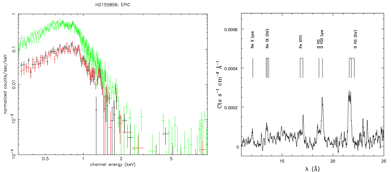
Fig. 1. Left: EPIC spectra of HD 155806 (pn data shown as the upper green curve, MOS data as the lower red and black curves). Right: Fluxed RGS spectrum of HD 155806 (from task RGSFLUXER , RGS1+2 , orders 1+2) with the main lines identified. The data were smoothed using a sliding box, to highlight the X-ray lines.
