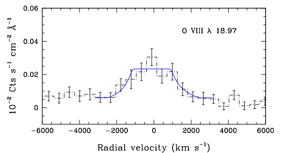
Fig. 2. The best-fit exospheric line-profile model (with the X-rays emitted above R_0 = 1.85 R_* and a wind opacity of \tau_{\lambda,*} = 0.0 ) overplotted on the RGS data of the O\text{ VIII Ly}\alpha line (binned to get 1000 bins for the entire wavelength range).
