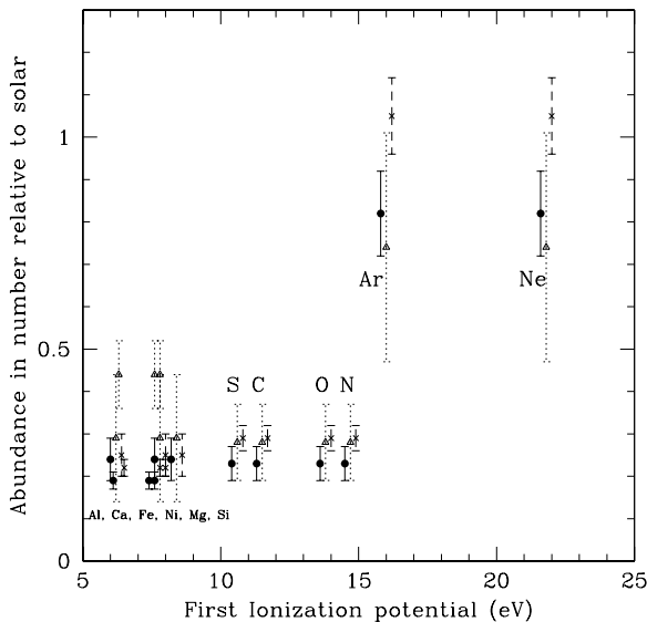
Fig. 5. The abundances of the elements, ordered by increasing FIP, derived from fits to the X-ray spectrum of 1RXS J171502.4–333344 (see Table 3). The values derived from EPIC+RGS fits are shown by filled circles, whereas the values associated with the quiescent and flaring phases are shown by open triangles and crosses, respectively (for clarity, they have been shifted right by 0.2 and 0.4 eV, respectively).
