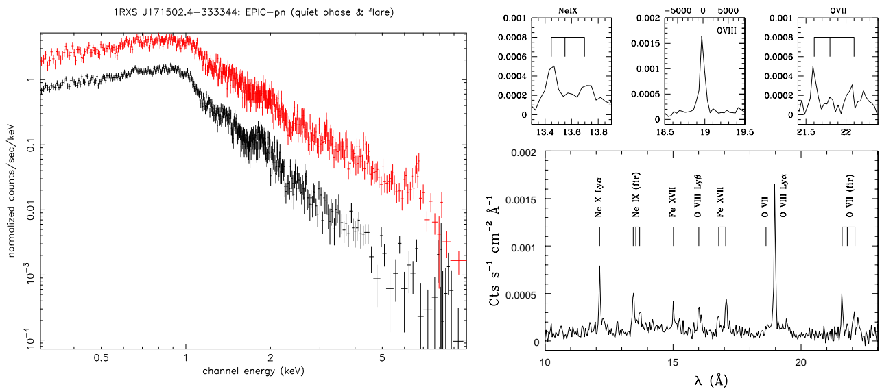
Fig. 4. Left: The EPIC-MOS2 spectra of 1RXS J171502.4–333344 (upper curve: during the flare, lower curve: in quiescence). Right: fluxed RGS spectrum.
