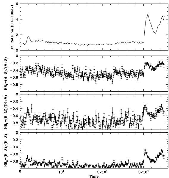
Fig. 3. The evolution of the EPIC-pn count rate (top) and hardness ratios for 1RXS J171502.4–333344, shown with a time bin of 200s.
