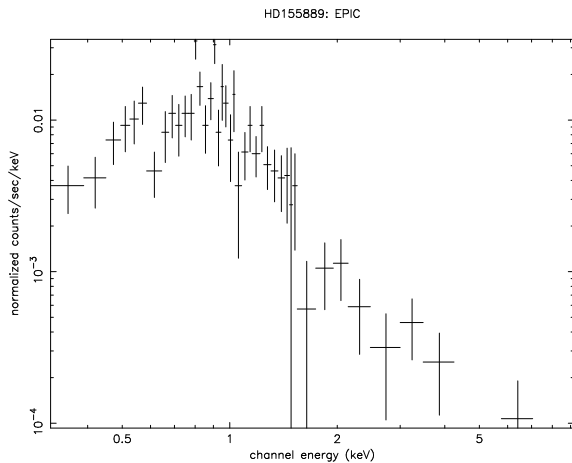
Fig. A.1. EPIC-MOS2 spectrum of HD 155889.
