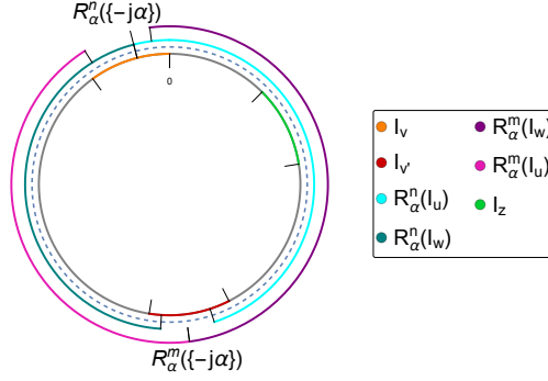
■ Figure 5 The situation depicted in the proof of Lemma 4.15.
