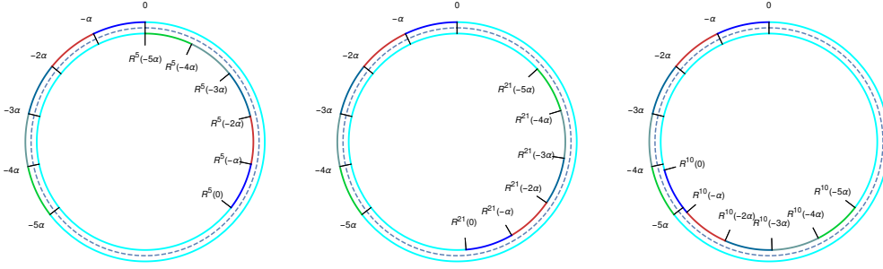
■ Figure 4 Constellations for \alpha = (\pi - 3)/2 , \ell = 5 , and n = 5, 21, 10 .
