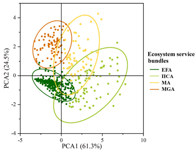
Fig. 5. Biplot of ES bundles for the first two PCA axes (85.8% of the variability absorbed). The color of labels indicates ecosystem services bundles and 95% confidence ellipses of bundles are added. Ecosystem services bundles are: EFA-Ecological fragile area; HCA-Habitat conservation area; MA-Multifunctional area; and MGA-Main grain-producing area).
