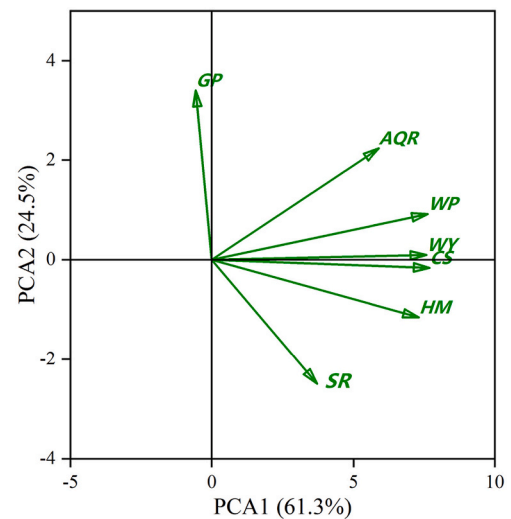
Fig. 3. Biplot of ecosystem services for the first two PCA axes (85.8% of the variability absorbed). ES indicators are: GP-grain production; WY-water yield; WP-water purification; SR-soil retention; CS-carbon storage; AQR-air quality regulation; and HM-habitat maintenance).
