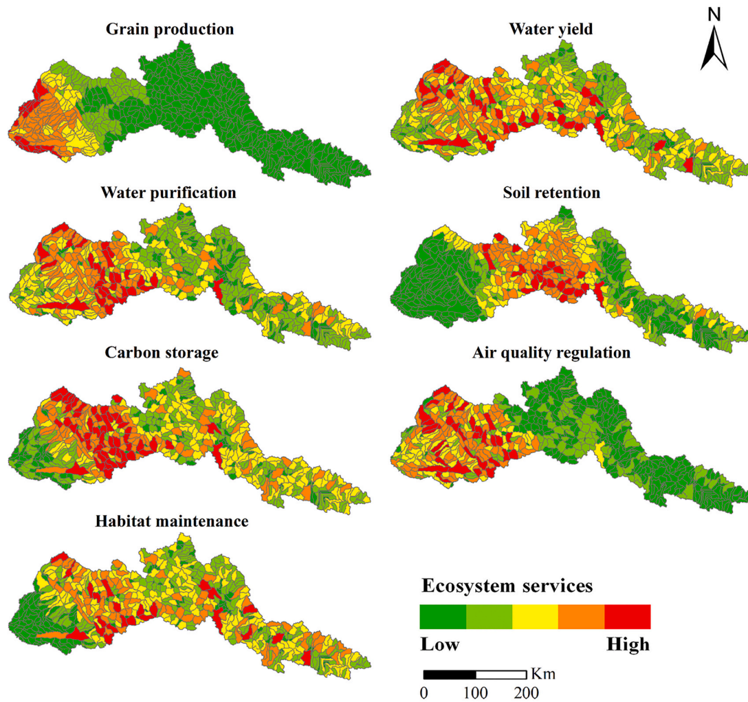
Fig. 2. Spatial patterns of ecosystem services provision in the Sutlej-Beas River Basin.
