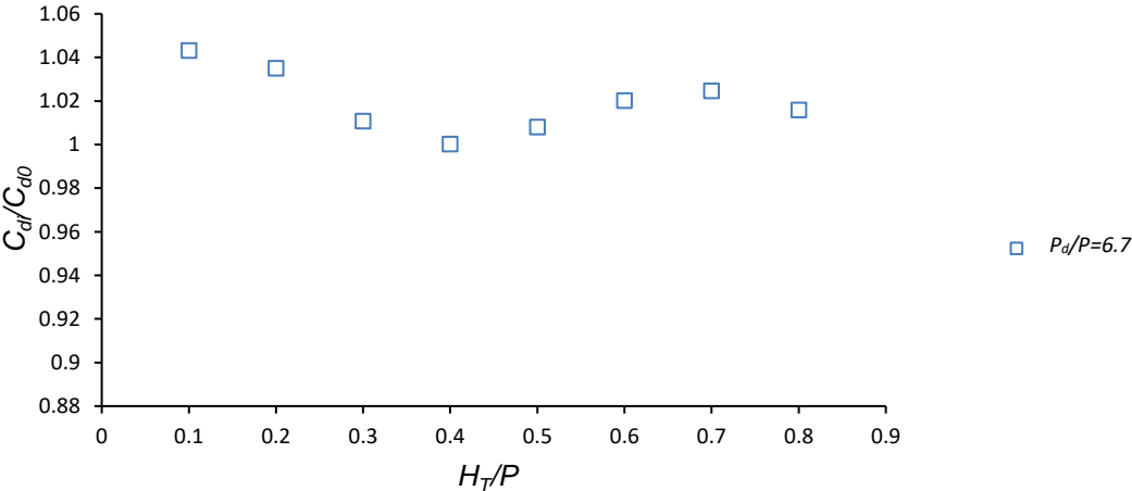
Figure 11 - Theoretical C_{dl}/C_{d0} ratio as a function of H_t/P for the PK weir.
