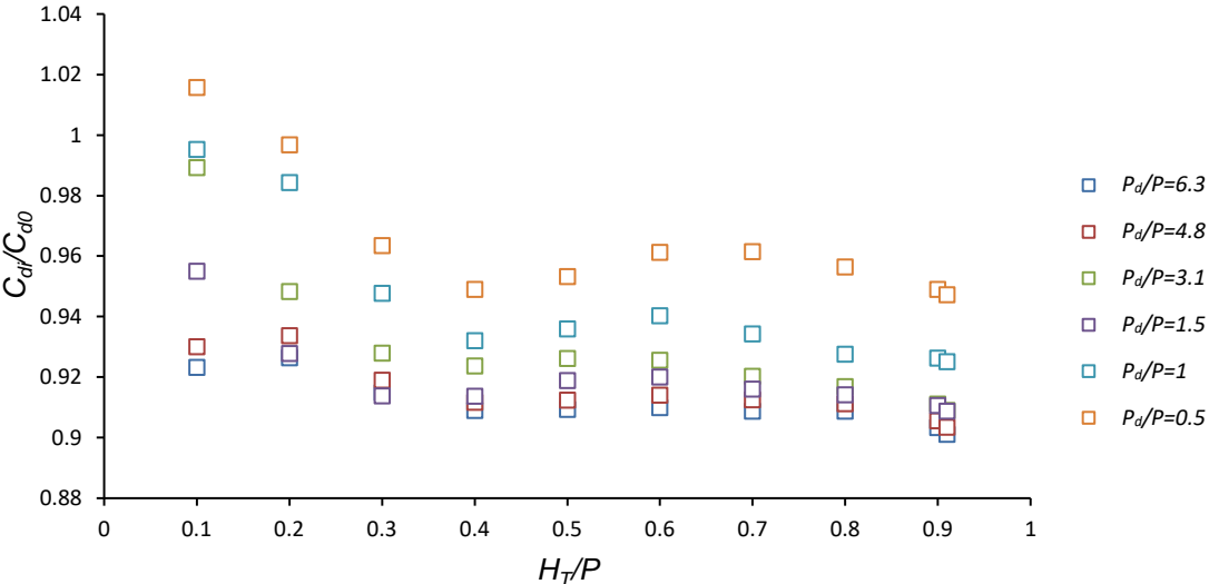
Figure 10 - Theoretical C_{dl}/C_{d0} ratio as a function of H_t/P for the labyrinth weir.
